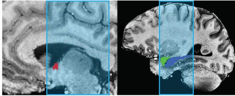
Figure 2. Example of BNST (red), Amygdala (green) and Hippocampus (blue) ROIs used to sample BOLD activity, after downsampling to EPI resolution. ROIs are overlaid onto anatomical scan, with coverage of partial brain EPI scan highlighted in light blue. BNST ROIs were drawn for each subject, according to the anatomical boundaries detailed by Avery et al. (2014). Amygdala and hippocampus ROIs were created using Freesurfer (v. 5.3.0, Martinos Center for Biomedical Imaging, Harvard-MIT, Boston, USA; Fischl et al., 2002).
