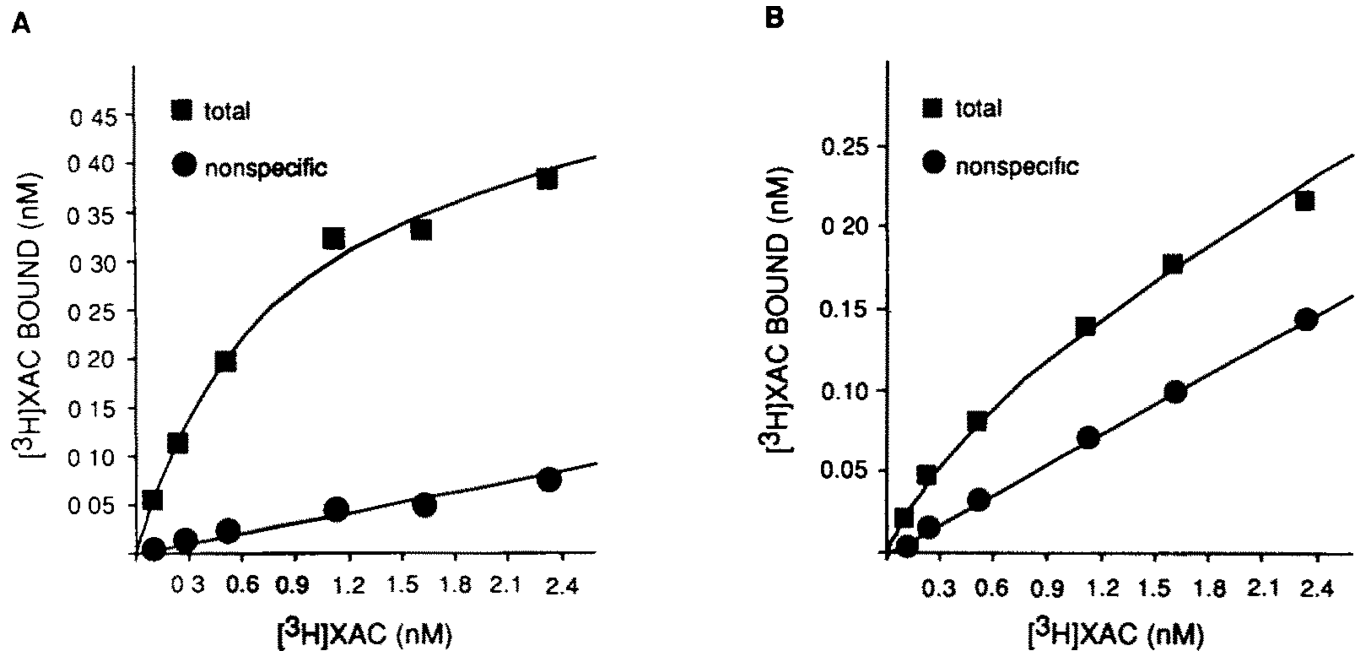
Fig.1. [^3\text{H}]\text{XAC} saturation curves in (A) solubilized bovine brain membranes and (B) XAC-Affi-Gel-purified preparation. Membrane solubilization, affinity chromatography and binding assays were performed as described in section 2. Non-specific binding was defined with 10 \mu\text{M} R -PIA or 5 \text{ mM} theophylline. Gpp(NH)p ( 10 \mu\text{M} ) was present in all assay tubes. These plots are representative of 5 similar experiments.
