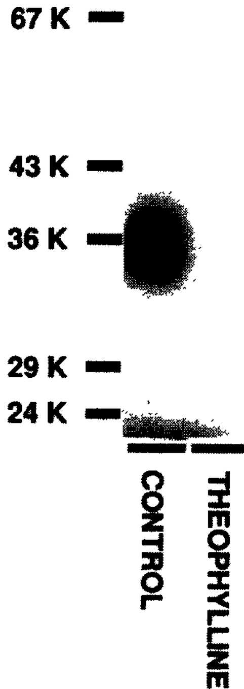
Fig.3. Photoaffinity labelling of XAC-Affi-Gel-purified A 1 adenosine receptor with [ 125 I]PAPAXAC-SANPAH. Chromatography and photoaffinity labelling were performed as described in section 2. Labelling was performed in the absence (control) or presence of 5 mM theophylline. Following labelling, the sample was solubilized in SDS and electrophoresed on a 12% acrylamide gel. The positions of iodinated molecular mass standards are shown to the left.
