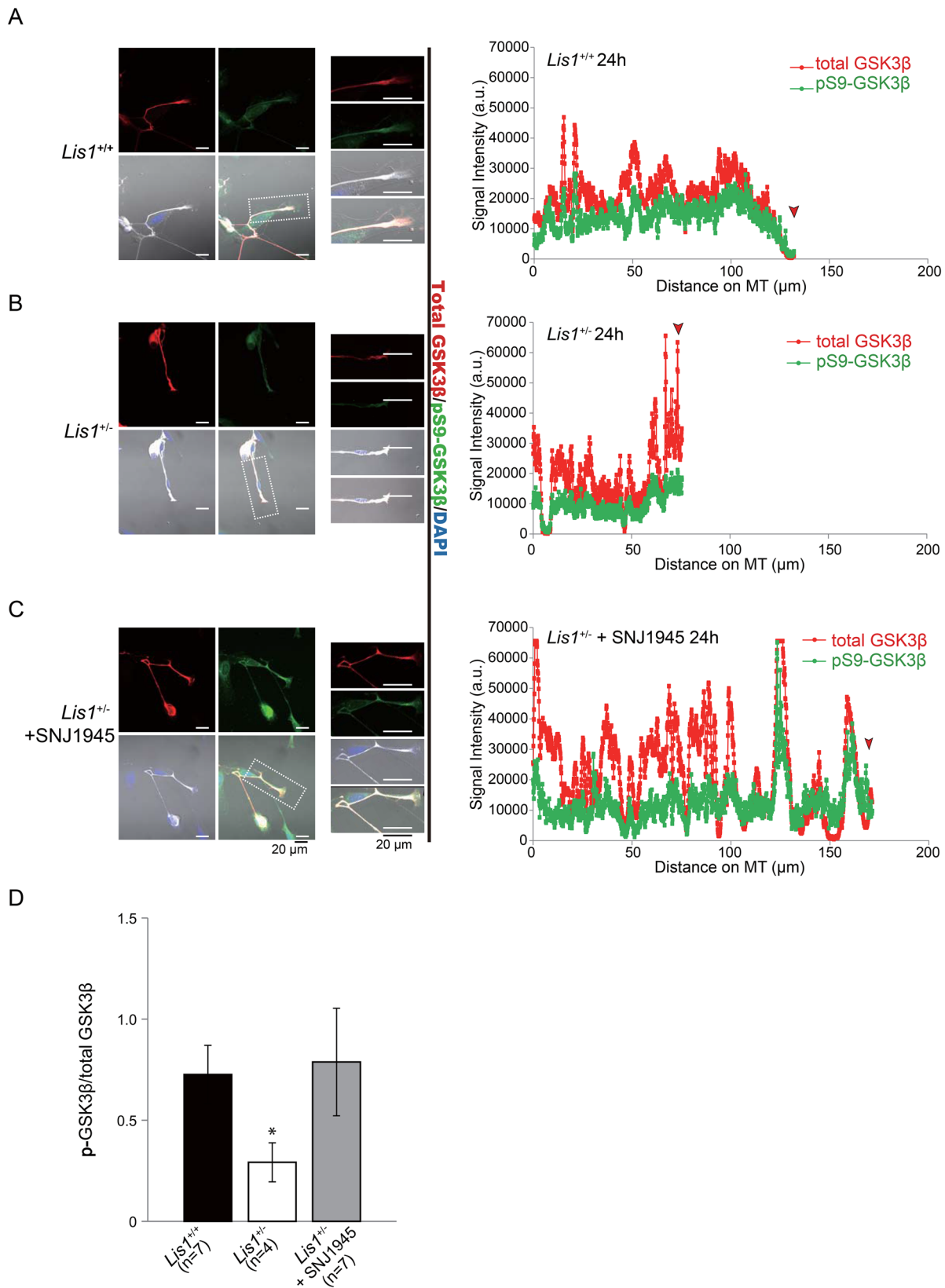
Fig. 5. Distribution of phospho-GSK-3 \beta (Ser9) in DRG neurons. (A-C) Left panels: DRG neurons from (A) Lis1 +/+ mice, (B) Lis1 +/- mice, and (C) SNJ1945-treated Lis1 +/- mice stained with anti-GSK-3 \beta (red), anti-pS9-GSK-3 \beta (green), and DAPI (blue). Middle panels: higher-magnification images of an area demarcated in the left panels (white boxes). Right panels: normalized fluorescence intensity along the axon. Red arrowheads indicate growth cones. Greater fluorescence intensity at the growth cones of DRG neurons from Lis1 +/+ (A) and SNJ1945-treated Lis1 +/- (C) mice indicates accumulation of total GSK-3 \beta and anti-pS9-GSK-3 \beta . (D) Quantitation of anti-pS9-GSK-3 \beta to total GSK-3 \beta intensity in growth cones indicates relatively lower accumulation of the inactive anti-pS9-GSK-3 \beta in Lis1 +/- growth cones and reversal by SNJ1945. *P<0.05 by ANOVA. Error bars indicate standard errors.
