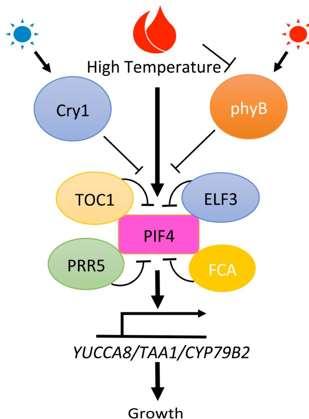
Figure 2. PIF4 plays a central role in integrating light and high temperature signaling to promote growth. High ambient temperature induces PIF4 expression and also stabilizes PIF4 protein. Multiple regulators have been shown to directly interact with PIF4 and regulate its function by inhibiting DNA binding, transcription activity and protein stability. While two photoreceptors, phyB and Cry1 function to inhibit PIF4 activity in response to red and blue light signals, respectively, only phyB has been shown to act as a thermosensor in Arabidopsis. PIF4 directly activates the expression of YUC/TAA1/CYP79B2 genes to promote growth.
