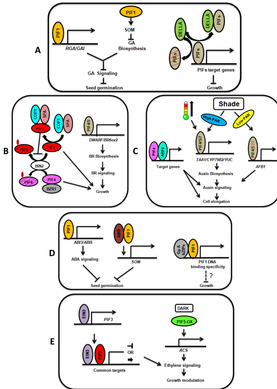
Figure 3. PIFs integrate light and hormone signaling pathways to modulate growth in Arabidopsis. (A, left) PIF1 has an exclusive role in regulating seed germination by directly activating RGA and GAI expression that inhibit GA signaling. PIF1 also inhibits GA biosynthesis indirectly by activating SOM expression, resulting in inhibition of seed germination in the dark. Light-induced degradation of PIF1 promotes seed germination. (Right) PIFs physically interact with DELLA proteins and this interaction results in inhibition of DNA binding activities of PIFs. DELLA proteins also induce degradation of PIFs in darkness and inhibit subsequent growth. (B, left) PIF4 interacts with BZR1 and regulates growth in response to BR and light signal. BIN2 phosphorylates PIF3 and PIF4 independent of light and promotes
