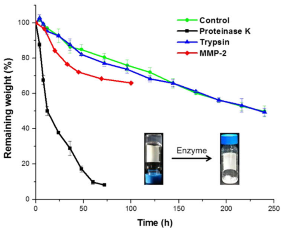
Figure 7. Weight loss profiles of hydrogels formed from polymer 1 in the presence and absence of enzymes. Measurements were repeated three times for proteinase K, trypsin and control group, and error bars represent the standard deviations. A single measurement was performed for MMP-2.
