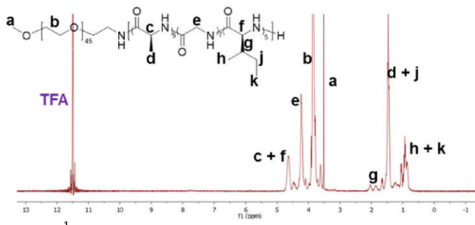
Figure 1. ^1\text{H} NMR spectrum of polymer 1 acquired in TFA-D.
