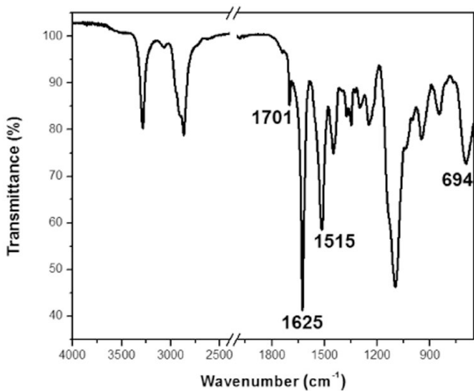
Figure 3. ATR-FTIR spectrum of polymer 1 in the solid state.
