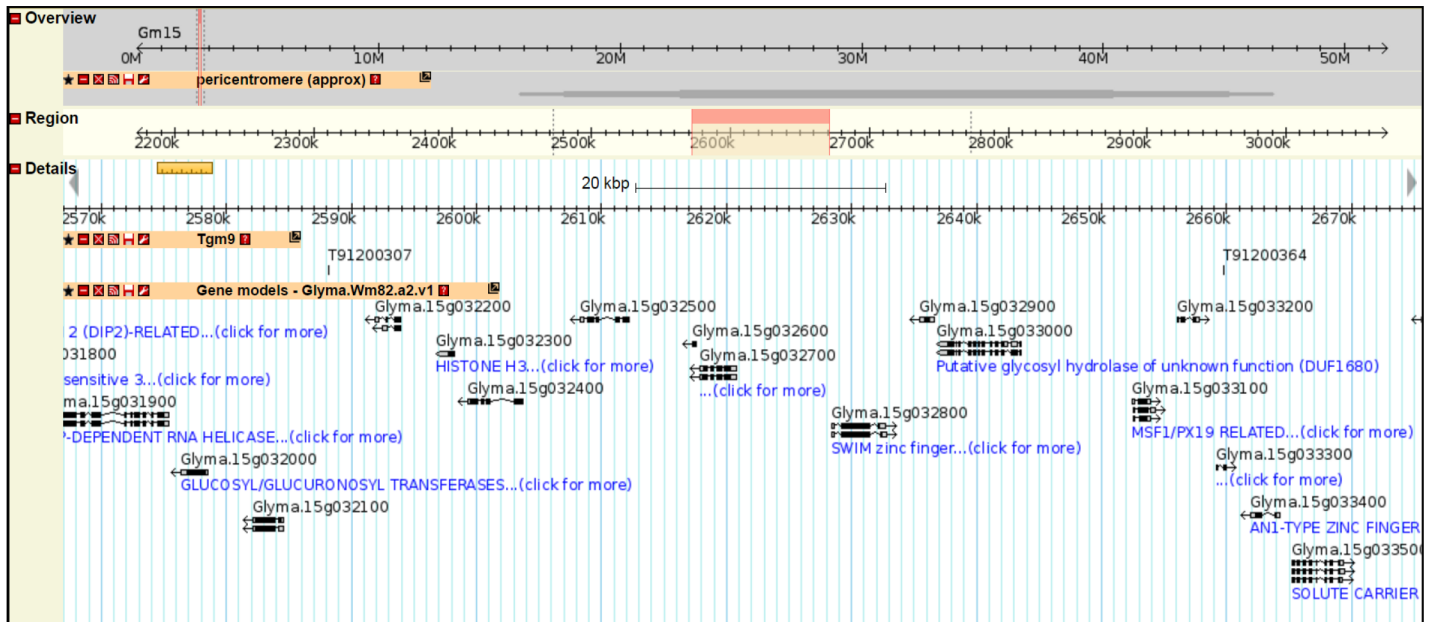
Fig 4. Display of Tgm9 -induced mutants in the SoyBase genome browser. The track for Tgm9 -insertion lines shows the location of two Tgm9 -induced insertions (T91200307 and T91200364) on Chromosome 15. Note that in the T91200307 mutant, the Tgm9 insertion site is located in the inter-genic region, and in T91200364, the insertion site is in the 2 nd exon of Glyma.15G033300 . ( http://soybase.org/gb2/gbrowse/gmax2.0x/?start=1;stop=56831624;ref=Gm01;width=1024;version=100;flip=0;grid=1;id=28f86f22137273c155fe3e1756259be0;l=tgm9-gene_models_wm82_a2_v1-pericentromere%3Aoverview {Please use user name: Bhatt; password: tgm9#}).
