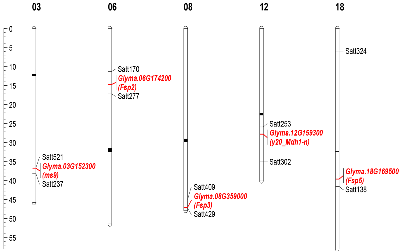
Fig 1. Physical map of five candidate genes that were mutated in Tgm9 -insertion mutants. Flanking molecular markers from the genetic linkage maps for y20 Mdh1-n , ms9 , Fsp2 , Fsp3 and Fsp5 were placed on the physical map along with Tgm9 -insertion sites identified in these mutants [29–31]. Scale is represented in million base pairs (Mb) of DNA.
