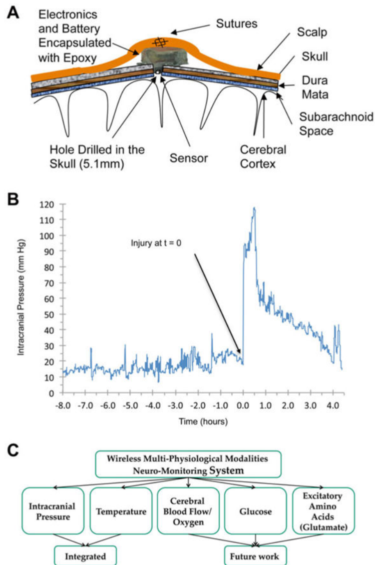
Fig. 6. Telemetry-based neuromonitoring system in swine model of closed-head rotational injury. (a) Schematic of implanted custom-built device contained above the skull with a burr hole for sensor access to CSF. (b) Example ICP trace from wireless device before and after closed-head TBI in swine. In this study, baseline ICP readings were relatively stable over the 8 h prior to injury at 16.7 \pm 4.6 mmHg (mean \pm standard deviation). We found that closed-head rotation TBI induced a rapid and extreme ICP spike occurring directly upon injury. The acute elevation in ICP generally lasted for 40–60 min, followed by a gradual decline to maintain a persistently elevated level over several hours post-injury. (c) Current and future capabilities of this fully implantable wireless neuromonitoring system
