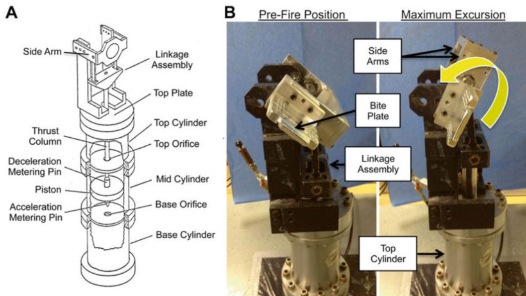
Fig. 4. HYGE device and custom-built linkage assembly for head rotation in the coronal plane. (a) Schematic of the HYGE pneumatic actuator and custom linkage assembly to convert the linear motion of the HYGE piston to angular motion. (b) Pictures of the HYGE device used to deliver head rotational acceleration in swine, demonstrating the pre-loading and maximum rotation position
