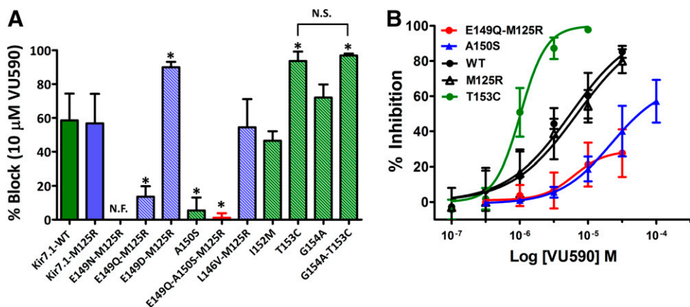
Fig. 3. Identification of pore-lining residues required for Kir7.1 inhibition by VU590. (A) Percent inhibition of Kir7.1-WT (solid green bar), Kir7.1-M125R (solid blue bar), and respective mutants (striped bars) by 10 \mu M VU590. (B) VU590 CRCs for Kir7.1-WT, Kir7.1-M125R, T153C, A150S, and E149Q-M125R mutants. Data were analyzed using one-way ANOVA with Bonferroni's multiple comparison test and plotted as mean \pm S.D. ( n \geq 5 ). * P < 0.05 , statistically significantly different from the respective control backgrounds (Kir7.1-WT or Kir7.1-M125R); N.F., nonfunctional; N.S., non-significant.
