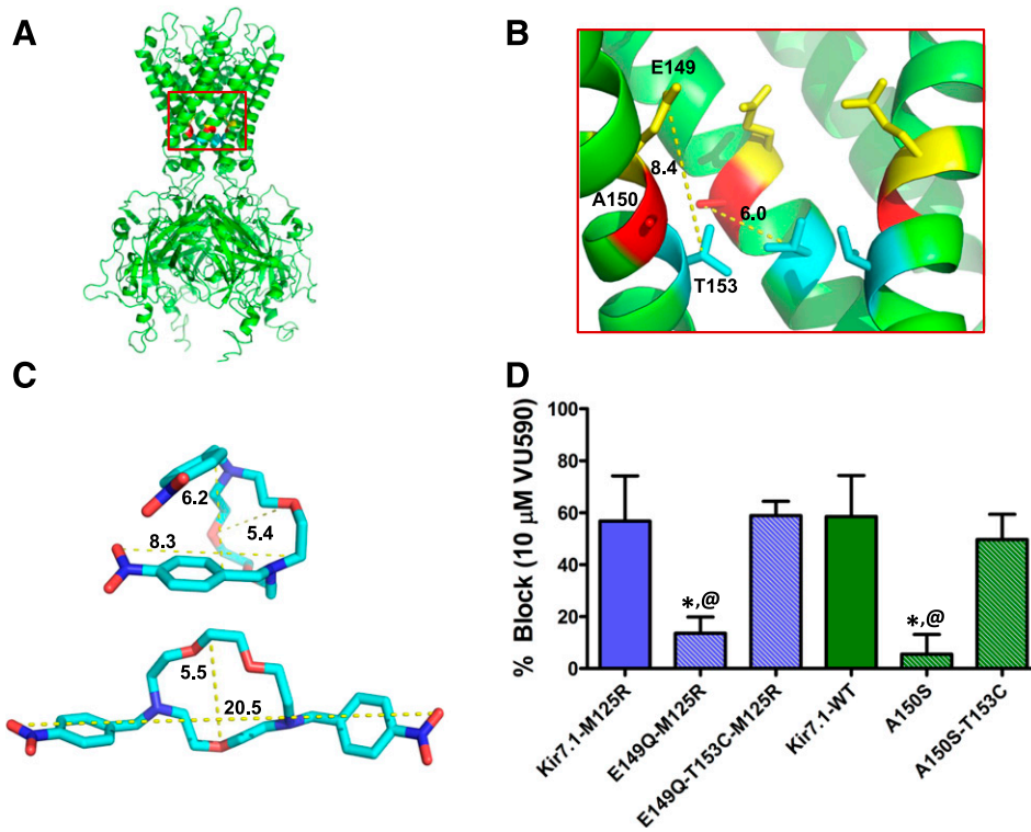
Fig. 5. The T153C mutation restores block of Kir7.1 binding-site mutants. (A) Kir7.1 homology model showing relative positions of E149, A150, and T153 residues. (B) Magnified section of the Kir7.1 homology model (red square in (A)) shows relative distances (in angstroms) between the E149 (yellow), A150 (red), and T153 (blue) residues. (C) Representative conformations of VU590 in either folded or extended states. (D) Mean \pm S.D. percent inhibition by 10 \mu M VU590. * P < 0.05, statistically significantly different from the respective control background (Kir7.1-WT or Kir7.1-M125R). Data were analyzed using one-way ANOVA with Bonferroni's multiple comparison test. @ P < 0.05 statistically significantly different from respective T153C mutants, n \geq 5 .
