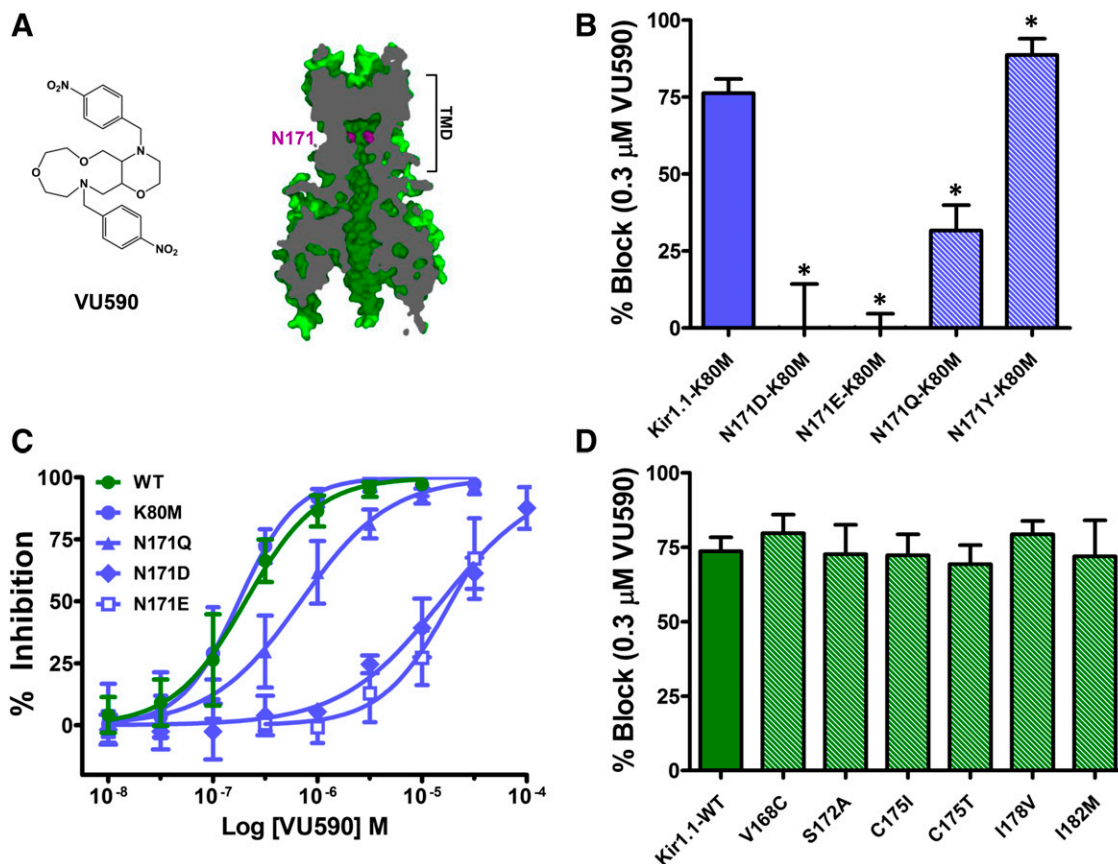
Fig. 1. N171 is required for VU590 block of Kir1.1. (A) (Left) Chemical structure of VU590. (Right) Section through a Kir1.1 homology model at the level of the pore showing the location of N171 (magenta), which is required for VU590 sensitivity. (B) Percent inhibition by 0.3 \mu\text{M} VU590 of Kir1.1-K80M (solid blue bar) and N171 mutants (striped bars). (C) VU590 CRCs for Kir1.1-WT (wild-type), K80M, N171Q, N171D and N171E mutants. (D) Percent inhibition of Kir1.1-WT (solid green bar) and respective mutants (striped bars) by 0.3 \mu\text{M} VU590. Data were analyzed using one-way ANOVA with Bonferroni's multiple comparison test and plotted as mean \pm S.D. percent inhibition ( n \geq 4 ); * P < 0.05 .
