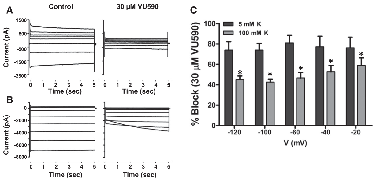
Fig. 2. Voltage and K^+ dependence of Kir7.1 block by VU590. Representative whole-cell current responses to voltage steps from a holding potential (A) -80 mV for 5 mM K^+ or (B) -7.5 mV for 100 mM K^+ in presence or absence of 30 \mu M VU590. (C) Mean \pm S.D. % inhibition by VU590 calculated at each voltage with 5 mM and 100 mM extracellular K^+ ( n = 4 ). * P < 0.05 compared with percent inhibition in 5 mM K^+ . Data were analyzed using two-way ANOVA with Bonferroni's multiple comparison test.
