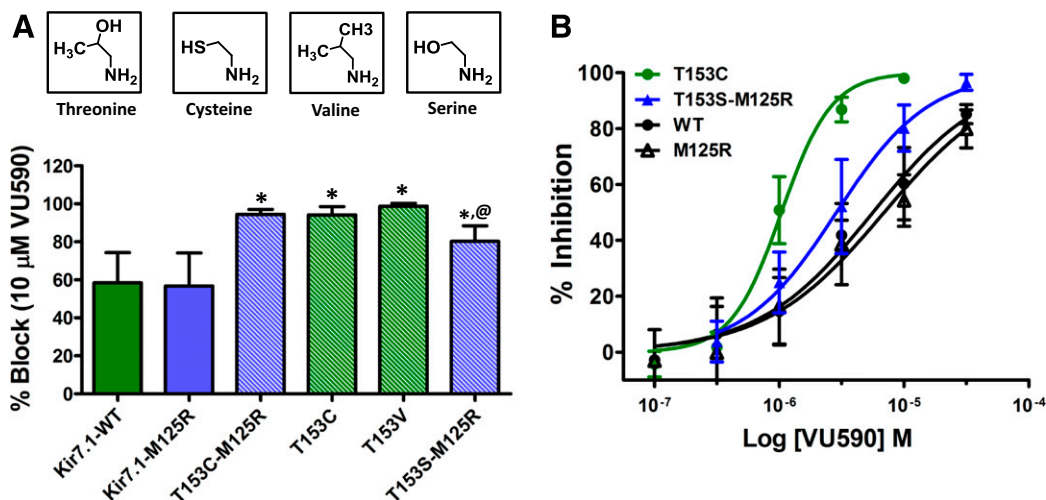
Fig. 4. Effect of mutations at position 153 on the sensitivity of Kir7.1 to VU590. (A) Mean \pm S.D. percent inhibition of Kir7.1-WT (solid green bar), Kir7.1-M125R (solid blue bar) channels and mutants (striped bars) by 10 \mu M VU590. (B) VU590 CRC comparison of Kir7.1-WT, Kir7.1-M125R, T153C, and T153S mutants. * P < 0.05 , statistically significantly different from the respective control background (Kir7.1-WT or Kir7.1-M125R). Data were analyzed using one-way ANOVA with Bonferroni's multiple comparison test. @ P < 0.05 , statistically significantly different from T153C and T153V mutants, n \geq 5 .
