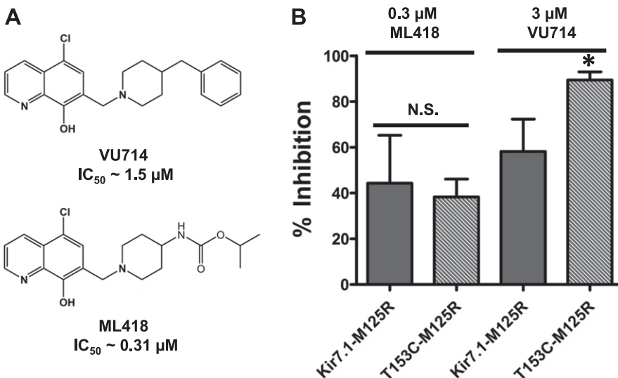
Fig. 6. T153C increases block by another low-affinity blocker, VU714. (A) Chemical structures of VU714 and ML418; (B) Mean \pm S.D. percent inhibition by 0.3 \mu M ML418 or 3 \mu M VU714 of M125R-T153C mutant. Data were analyzed using unpaired t test. * P < 0.05 statistically significantly different from the respective control background (Kir7.1-M125R), n \geq 5 . N.S., non-significant.
