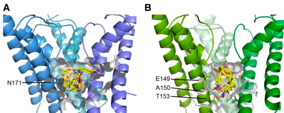
Fig. 8. VU590 binds to Kir1.1 and Kir7.1 using different binding modes. (A) Model of VU590 bound to Kir1.1 using three shades of blue (the fourth chain is hidden for clarity), with the pore cavity highlighted by a transparent gray surface. The best-scoring five poses of VU590 are shown as sticks, where yellow is carbon, blue nitrogen, and red oxygen. The side chain of residue N171 is shown on the three subunits. (B) Model of VU590 bound to Kir7.1 as above but in green. The side chains of residues E149, A150, and T153 are shown.
