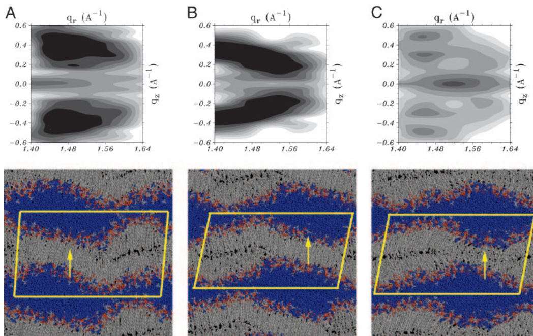
Fig. 3. Calculated WAXS intensities from ( Upper ) and snapshots of ( Lower ) DPPC ripple structures. The intensity is plotted as contours colored on a gray scale, using logarithmic procession of the levels. The levels are the same in all pictures, and the intensities were calculated from the positions of the same number of atoms. In the snapshots, Corey, Pauling, Kultun coloring is used, except for water, which is colored blue. The yellow lines show the projection of the unit cell on the x - z plane and the arrow indicates the z axis. (A) Ripple phase structure. (B) Ripple-like structure after partial melting of the M domain. (C) Ripple-like structure with an ordered M domain and liquid-like m domain.
