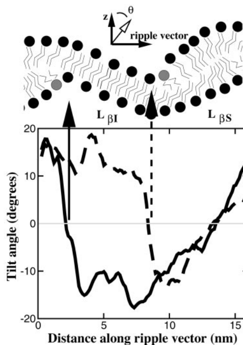
Fig. 4. Tilt of lipids in the ripple phase. ( Upper ) A schematic representation of the organization of the lipids in the ripple structure. ( Lower ) The tilt angle of the tails of the lipids with respect to the overall ripple normal (the z axis) is shown as a function of position along the ripple vector. The tilt angles of the chains in the two leaflets of the bilayer are shown separately. The dotted line corresponds to the upper leaflet; the drawn line corresponds to the lower leaflet. Clearly shown are the reversal of the tilt angle along the ripple vector in each monolayer at one end of the kink region (indicated by arrows) and the splay in the gel-like domain (gradual change in tilt angle between 10 and 16 nm). The parallel arrangement of the chains in the interdigitated region (between 3 and 8 nm) is also clearly visible. The tilt angle is defined as the angle between the vector connecting the fourth and 12th carbon atoms in each DPPC tail and the z axis. The data are calculated from a representative simulation of the DPPC ripple phase.
