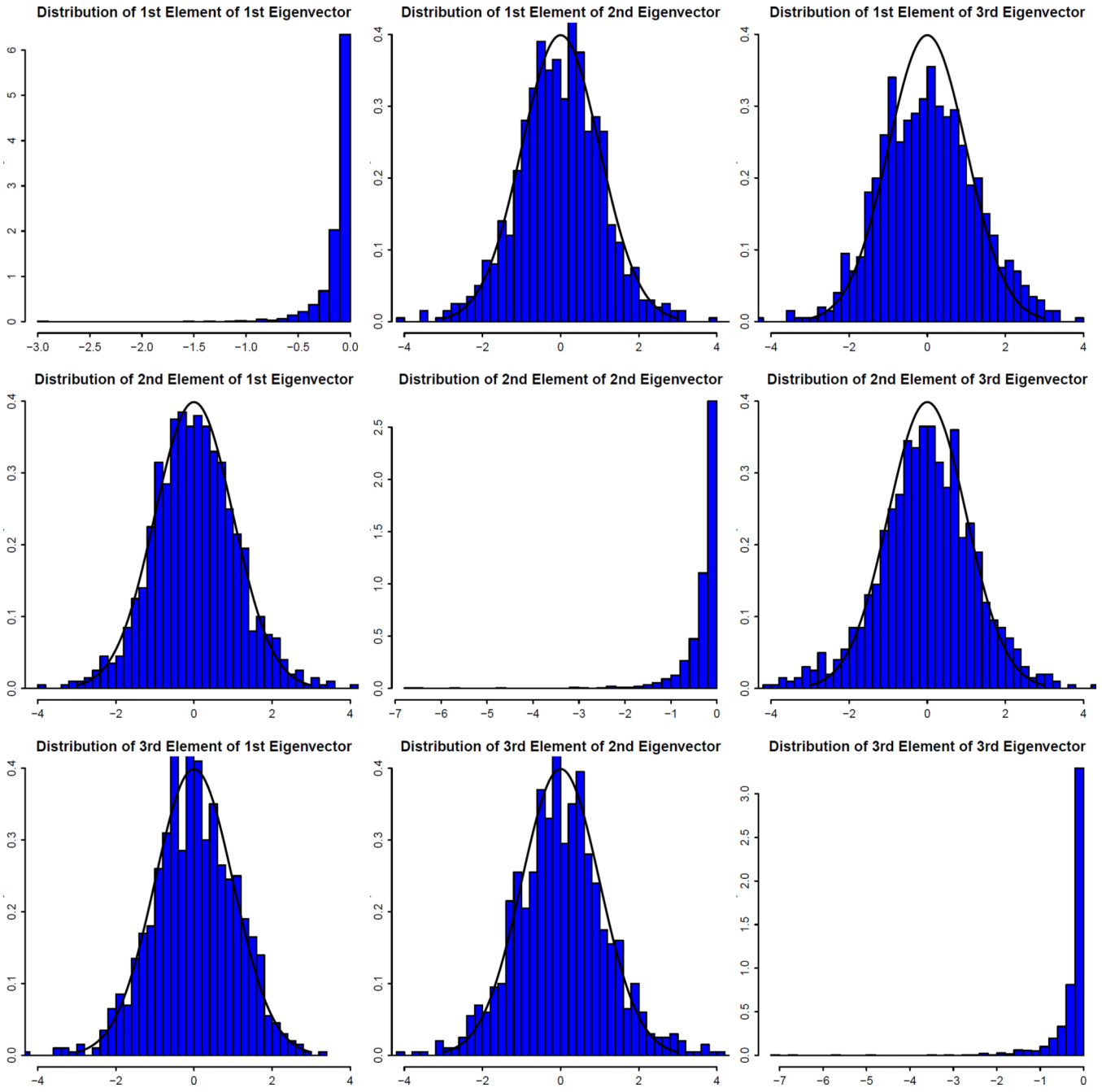
Fig 2. Behavior of empirical eigenvectors. The histogram of the k^{th} element of the j^{th} empirical vector is depicted in the location (k, j) for k, j = 1, 2, 3 . Off-diagonal plots of values \sqrt{n}\hat{\xi}_{jk}/\|\hat{\xi}_{jA}\|/\sqrt{\frac{c_j c_k}{(c_j - c_k)^2}} are compared to their asymptotic distributions N(0, 1) for k \neq j while diagonal plots of values \sqrt{n}(\hat{\xi}_{jj}/\|\hat{\xi}_{jA}\| - 1) are compared to stochastically 0.
