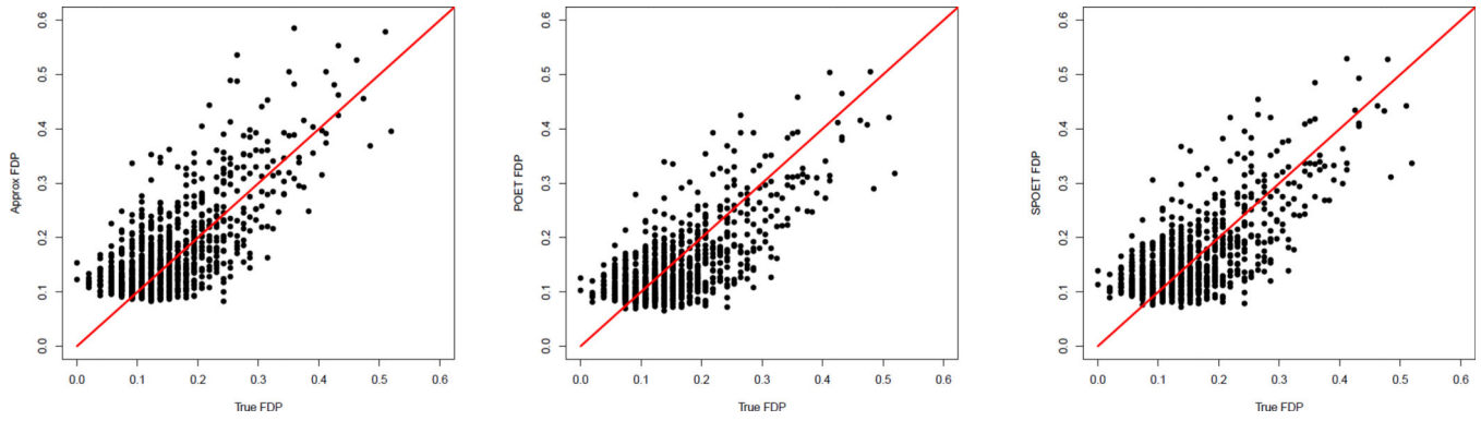
Fig 6. Comparison of estimated FDP's with true values. The left plot assumes knowledge of B , the middle and right ones are corresponding to POET and S-POET methods respectively. The results are aligned along the 45-degree line, indicating the accuracy of the estimated FDP.
