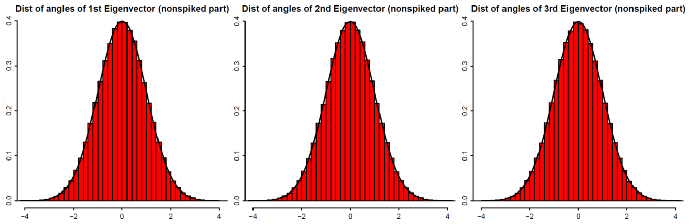
Fig 3. The empirical distributions of all pairwise angles of the 1000 realized \hat{\xi}_{jB}/\|\hat{\xi}_{jB}\| ( j = 1, 2, 3 ) compared with their asymptotic distributions N(0, 1) .
