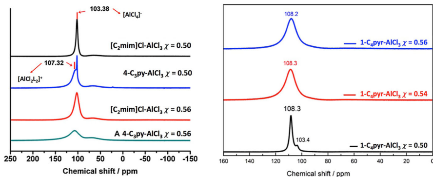
Fig. 11 Comparison of 27 Al NMR spectra. Left ionic liquid, [C 2 mim]Cl-AlCl 3 , and an LCC, 4-C 3 py-AlCl 3 , at two molar ratios of aluminium(III) chloride: \chi_{\text{AlCl}_3} = 0.50 and 0.56 . Right 1-C 4 pyr-AlCl 3 , at three molar ratios of aluminium(III) chloride: \chi_{\text{AlCl}_3} = 0.50, 0.54 and 0.56 . Left Adapted from [163]. Right Adapted from [165]
