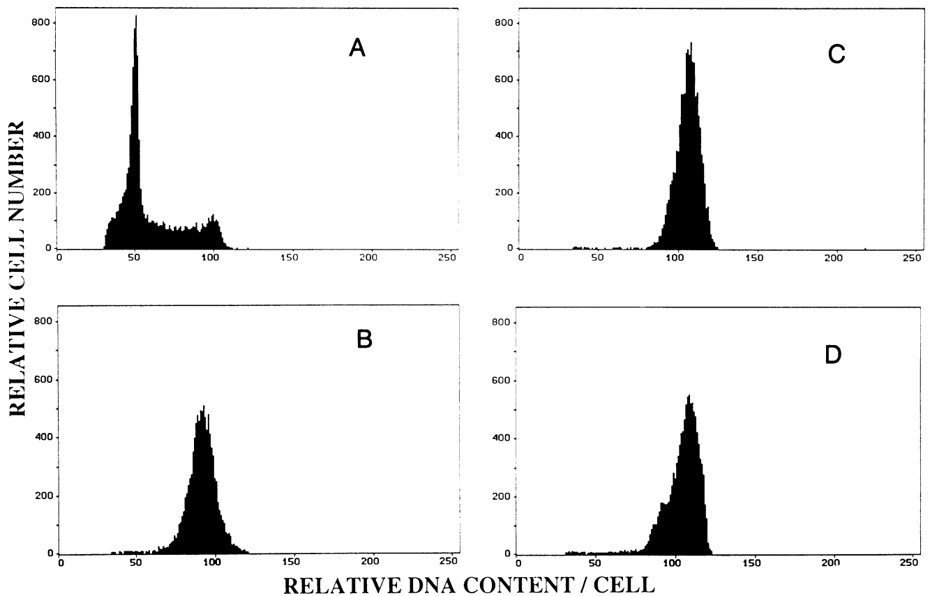
Fig. 1. Cell cycle analysis of proliferating and \gamma -irradiated HeLa CD4-LTR/ \beta -gal cells. The abscissa is the relative DNA content per cell, while the ordinate is the cell number. (A) Logarithmically growing cells; (B) cells 24 h after exposure to 4000 rads; (C) 48 h after exposure to 4000 rads; (D) 72 h after exposure to 4000 rads.
