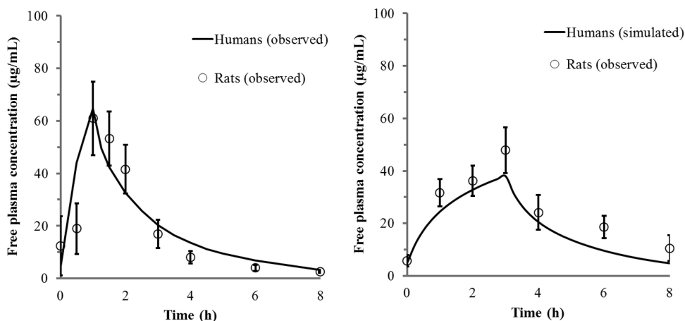
FIG 1 Free-drug concentration-time profiles in plasma for a 1-h infusion (left) or a simulated 3-h infusion (right) of 2 g cefiderocol in humans and rats. Each open circle represents the mean; error bars, standard deviations ( n = 8 ). PK profiles in humans and rats were derived from healthy humans and infected rats (left) or from simulated humans and infected rats (right).
