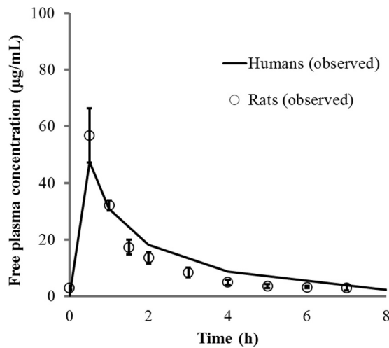
FIG 2 Free-drug concentration-time profiles in plasma for a 0.5-h infusion of 1 g ceftazidime in humans and rats. Each open circle represents the mean; error bars, standard deviations ( n = 5 ).
