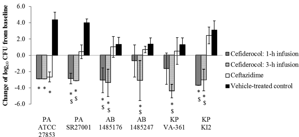
FIG 3 Efficacy of cefiderocol and ceftazidime against test isolates in rat respiratory tract infection models recreating human plasma PK. Data represent means \pm standard deviations of results from 4 to 7 rats. The symbols below the bars indicate significant differences ( P < 0.05 ) from the baseline control value (*) or from the result for ceftazidime ($) by Welch's t test. PA, Pseudomonas aeruginosa ; AB, Acinetobacter baumannii ; KP, Klebsiella pneumoniae .
