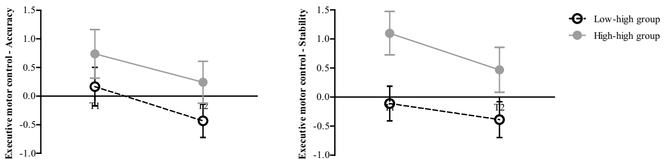
Fig. 2 Executive motor control: accuracy and stability of movement. Time effect was significant for accuracy and stability: all participants improved over time. Group effect was significant for stability only:
