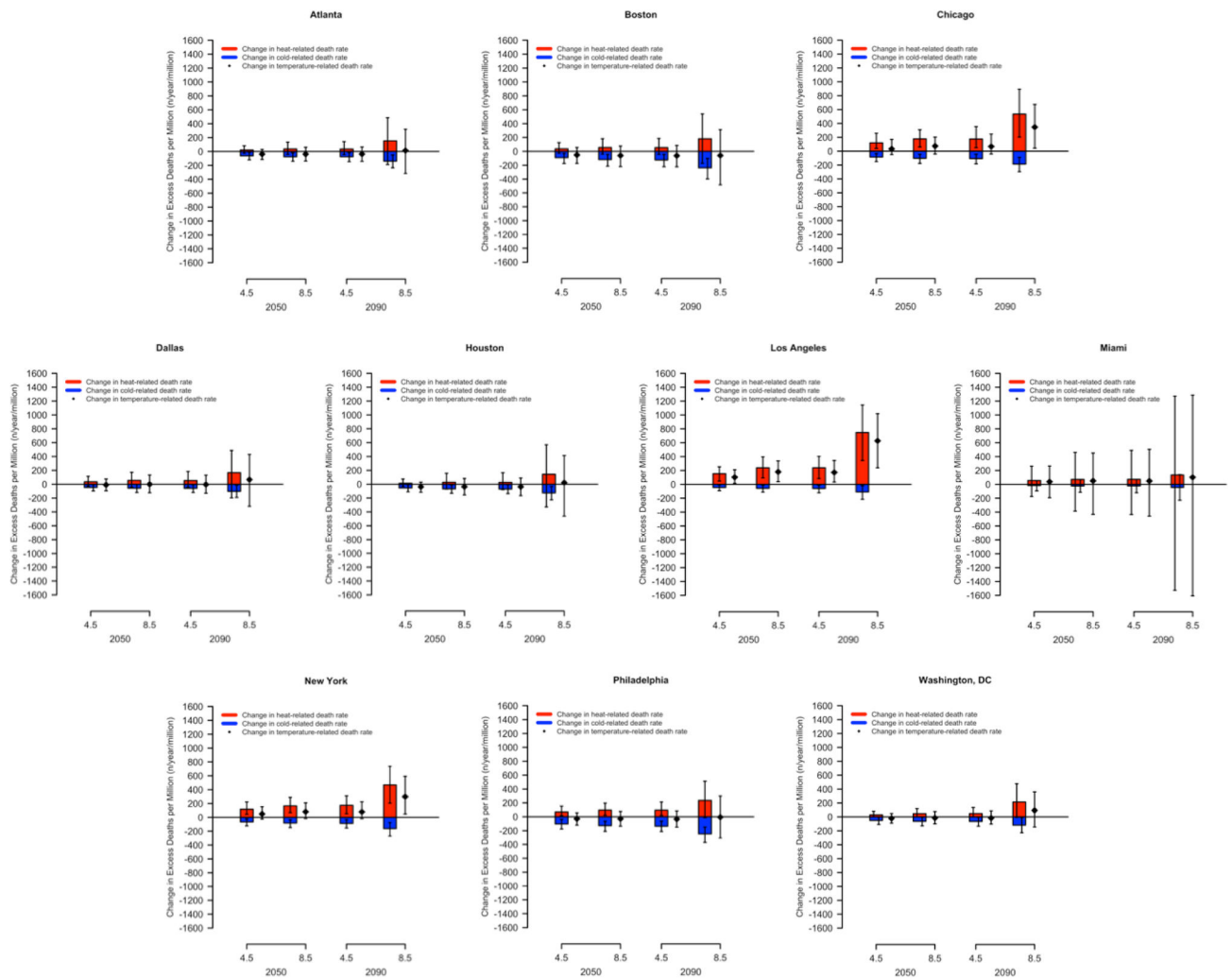
Figure 2. Projected change in the annual heat-related, cold-related, and total temperature-related mortality rate in each of 10 metropolitan areas in two future decades (centered at 2050 and 2090) and under two representative concentration pathways (RCP 4.5 and 8.5).
