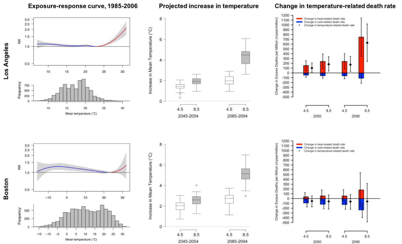
Figure 1. Exposure-response curves characterizing the present-day relationship between mean daily temperature and mortality (left), increase in mean daily temperature projected by the CMIP5 model ensemble (middle), and projected change in the annual heat-related, cold-related, and total temperature-related mortality rate per million people in the Los Angeles and Boston metropolitan areas in 2050 and 2090 and under two representative concentration pathways (RCP 4.5 and RCP 8.5, right).
