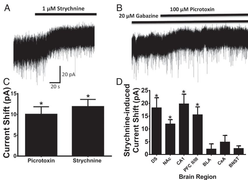
Fig. 2. Endogenous tonically activated GlyR currents in brain. ( A ) To identify tonic GlyR currents in MSNs in the nucleus accumbens, the effects of 1 \mu M strychnine on baseline holding currents were measured. ( B ) To determine whether tonic GlyR currents are due to activation of \alpha homomers, the effects of 100 \mu M picrotoxin (in the presence of gabazine) on baseline holding currents were determined. ( C ) Strychnine induced significant shifts in the holding current of MSNs [ t(42) = 6.872 , P < 0.0001 ], indicating the presence of a tonic GlyR conductance. Similarly, picrotoxin applications induced significant shifts in holding currents [ t(5) = 5.52 , P = 0.003 ]. The amplitudes of the current shifts induced by strychnine and picrotoxin were not significantly different from each other [ t(47) = 0.39 , P = 0.70 ]; n = 6 –43 neurons from 3–18 mice. ( D ) To identify tonic GlyR currents in each of the brain regions in which exogenous glycine-activated currents were detected, the effects of 1 \mu M strychnine on baseline holding currents were measured. Significant strychnine-induced shifts in holding current were detected in the dorsolateral striatum (DS) [ t(17) = 4.59 , P = 0.0003 ], NAc [ t(42) = 6.87 , P < 0.0001 ], hippocampus (CA1) [ t(6) = 5.12 , P = 0.0022 ], and PFC (layer II/III) [ t(11) = 4.97 , P = 0.0004 ], indicating the presence of tonic GlyR currents in these regions. In contrast, there was no effect of strychnine on the holding current of neurons recorded from the basolateral amygdala (BLA) [ t(9) = 1.00 , P = 0.34 ], central nucleus of the amygdala (CeA) [ t(6) = 1.82 , P = 0.12 ], or BNST [ t(10) = 2.15 , P = 0.06 ], indicating the absence of tonic GlyR currents in these regions. Data are presented as means \pm SEM ( n = 7 –43 neurons from 5–18 mice); * P < 0.05 .
