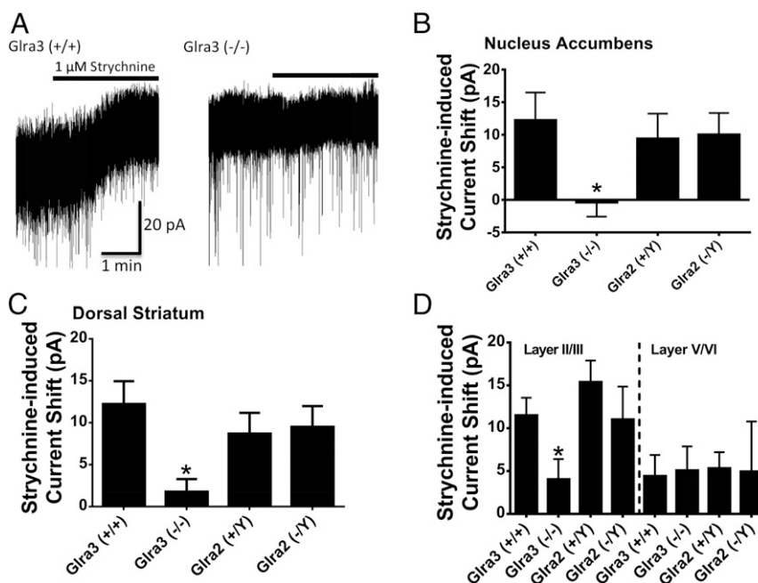
Fig. 3. Tonic GlyR currents in forebrain are mediated by \alpha 3 subunit-containing GlyRs. The effects of strychnine on baseline holding currents were measured and compared in Gla2 -Y and Gla3 -/- mice and their WT littermates. Whole-cell recordings were performed in the striatum and PFC, regions in which significant tonic GlyR currents were identified in C57/BL6J mice. (A) Sample tracings demonstrating the effects of 1 \mu M strychnine on the holding currents of MSNs in the NAC of Gla3 +/+ (Left) and Gla3 -/- (Right) mice. (B and C) Strychnine-induced shifts in the holding currents of MSNs in the NAC ( n = 4 –10 cells from three to seven mice) (B) and dorsal striatum ( n = 6 –9 cells from four to six mice) (C) of Gla3 +/+ mice, indicating the presence of a tonic GlyR current [NAC: t(14) = 2.93 , P = 0.011 ; dorsal striatum: t(11) = 3.58 , P = 0.004 ]; however, no significant shift was observed in Gla3 -/- mice. Strychnine-induced shifts in holding current were detected in MSNs in the NAC (B) and dorsal striatum (C) of both Gla2 +Y and Gla2 -Y mice. The amplitude of the tonic GlyR current was not significantly different between the two genotypes in either region of the striatum [NAC: t(10) = 0.12 , P = 0.91 ; dorsal striatum: t(16) = 0.24 , P = 0.81 ]. (D) In the medial prefrontal cortex, applications of 1 \mu M strychnine produced shifts in the holding currents of layer II/III pyramidal neurons in Gla3 +/+ mice; however, as in the striatum, this effect of strychnine was absent in neurons from Gla3 -/- mice [ t(15) = 2.40 , P = 0.029 ]. GlyR tonic currents were detected in neurons recorded from both Gla2 +Y and Gla2 -Y mice, and the amplitude of the strychnine-induced currents was not significantly different between the genotypes [ t(15) = 0.97 , P = 0.35 ]. In contrast to layer II/III, there were no significant effects of strychnine on the baseline holding currents of pyramidal neurons in layer V/VI in any of the mouse genotypes tested, suggesting the lack of an appreciable tonic GlyR current in this cortical layer. Data represent means \pm SEM ( n = 6 –9 neurons from three to seven mice; * P < 0.05 compared with WT littermates).
