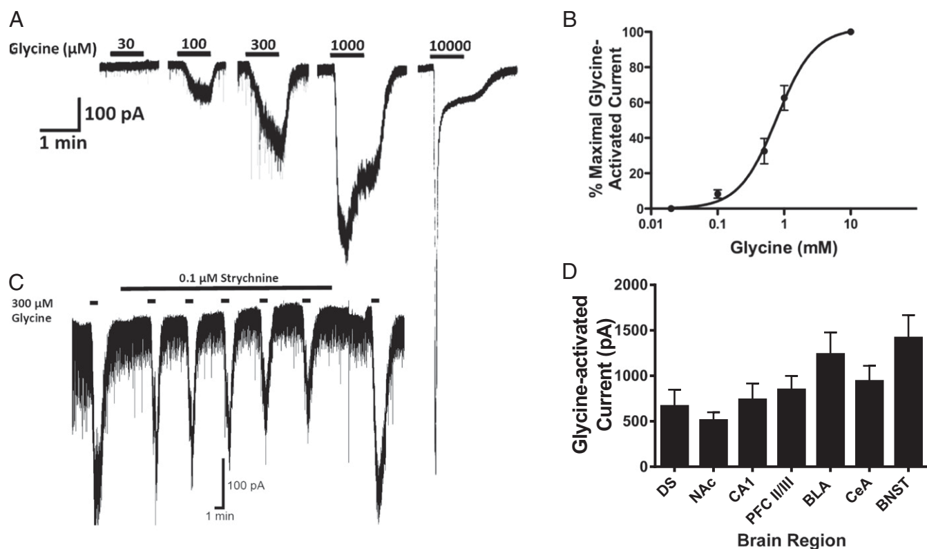
Fig. 1. Exogenous glycine-activated GlyR currents in the forebrain. ( A and B ) Whole-cell currents elicited by exogenous glycine applications (30 \mu M–10 mM) were recorded from MSNs in vitro in the NAc ( A ), and glycine concentration–response curves were generated ( B ), confirming the presence of measurable glycine-activated currents. ( C ) To demonstrate that the currents measured in A and B were due to glycine action at strychnine-sensitive GlyRs and not other neurotransmitter receptors, whole-cell currents elicited by glycine were first measured in the absence and then in the presence of a concurrent application of the GlyR-specific antagonist strychnine (100 nM). The amplitude of current produced by applications of 300 \mu M glycine was reduced in the presence of strychnine. ( D ) Currents elicited by 1 mM glycine were measured in several brain regions. Glycine-activated currents were present in the dorsolateral striatum (DS), NAc, hippocampus (CA1), layer II/III of the medial PFC, basolateral amygdala (BLA), central nucleus of the amygdala (CeA), and the BNST. Data represent means \pm SEM ( n = 8 –26 neurons from 7–11 mice).
