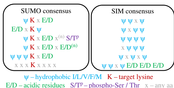
Figure 2. SUMO and SIM consensus (adapted from [10]). SUMO conjugation sites (left) are often found within the consensus \psi KxE/D where \psi is a hydrophobic amino acid and x is any amino acid. Several variants including an inverted variant, and variants with additional acidic patches of amino acids or phosphorylated Ser/Thr residues have been identified. Approximately 25% of SUMO sites do not conform to any consensus [11]. Hydrophobic SUMO Interacting Motifs (SIMs) (right).
