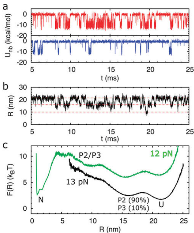
Fig. 3. Coarse-grained pulling simulations for the pbuE A-riboswitch using MD generated structures. (a) The time traces of non-bonded energies of helices P2 (red line) and P3 (blue line) in a trajectory showing that P2 spends more time in the folded state than P3 for the pbuE A-riboswitch aptamer at f=13 pN. (b) The time traces of the end-to-end distance, R , of the riboswitch for the trajectory in (a). (c) The free energy profile obtained based on the time traces for f=12 (green line) and 13 pN (black line). Interestingly, when f is increased by 1 pN from f=12 to f=13 pN the folded state is completely destabilized.
