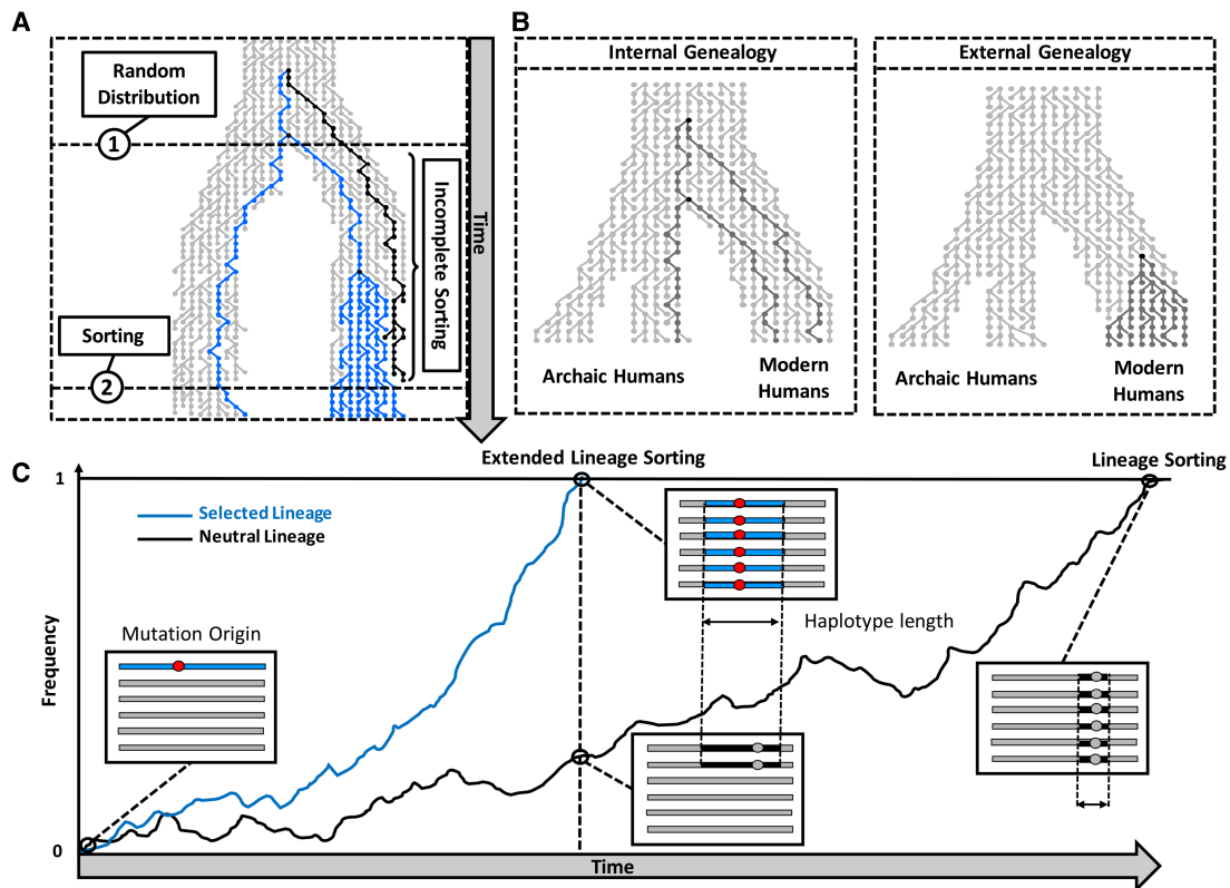
Figure 1. Illustration of the lineage sorting process. (A) Effects on the genealogy. The process starts with a random distribution of lineages when the ancestral population splits. The lineage in black is an outgroup to lineages in blue, so that the blue lineages show a closer relationship between populations than to the black lineage (incomplete lineage sorting). When the blue lineages in the top population reach fixation (through a selective sweep for instance), any lineage from the other populations will constitute an outgroup, thereby completing the sorting of lineages. (B) Two types of genealogies illustrating the possible relationships between an archaic lineage and modern human lineages. (C) Local effects in the genome at different time points. The curves represent the progression of lineage sorting for two independent regions, evolving under neutrality (black curve) and positive selection (blue curve), respectively. Longer fixation times are associated with more recombination so that neutrality produces smaller external regions.
