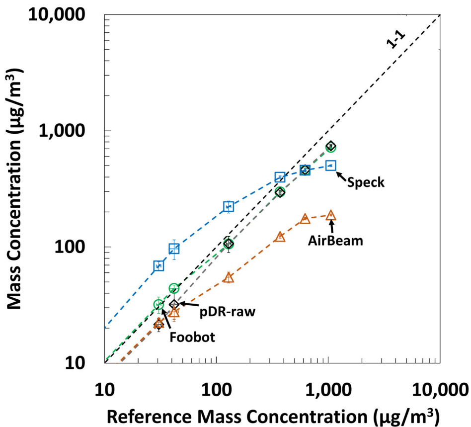
Figure 4. Mass concentrations measured by consumer air quality monitors and the pDR-raw (uncorrected mass) relative to reference mass concentration for ARD aerosol. The error bars represent one standard deviation.
