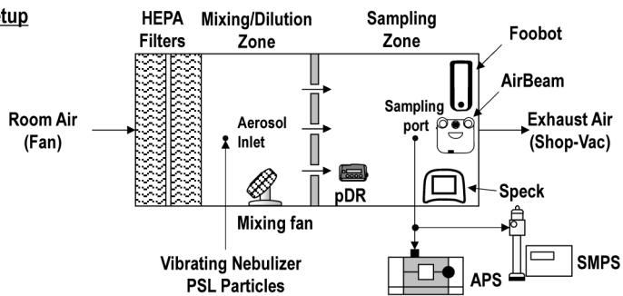
Figure 1. Experimental set up used to determine the performance of the CAMs
