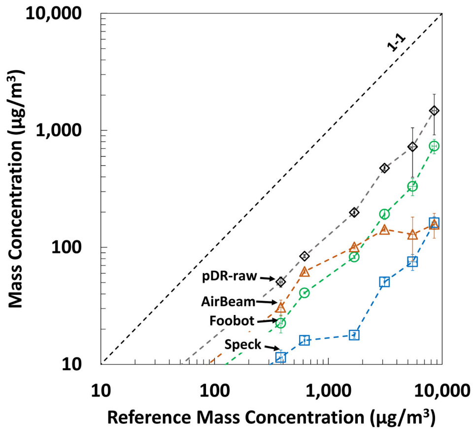
Figure 3. Mass concentrations measured by consumer air quality monitors and the pDR-raw (uncorrected mass) relative to reference mass concentration for welding aerosol. The error bars represent one standard deviation.
