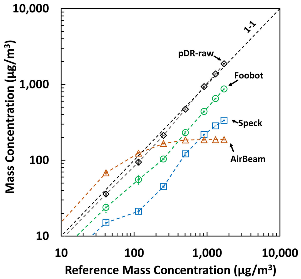
Figure 2. Mass concentrations measured by consumer air quality monitors and the pDR-raw (uncorrected mass) relative to reference mass concentration for salt aerosol. The error bars represent one standard deviation.
