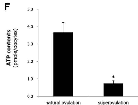
Fig. 4. Deformity and functional activity of mitochondria in mature (metaphase II stage) oocytes retrieved after superovulation treatment or natural ovulation. (A) (natural ovulation) and (B) (superovulation) show morphological difference of mitochondria. Confocal images of mitochondria in oocytes retrieved from natural ovulation (C) or superovulation after JC-1 staining (D). (E) Statistical comparison of mitochondrial activity (mean \pm SE) with using of confocal images. Significant ( p = 0.0179 ) difference between two treatments. (F) Quantitative comparison of ATP generation (mean \pm SE) in oocytes retrieved from after superovulation or retrieved from natural ovulation. Significantly ( p = 0.0002 ) different. Arrowhead, Well-developed mitochondrial cristae; asterisk, vacuolated mitochondria; F, Filament; L, Lipid droplet; M, Mitochondria. Magnification = \times 12,000 . Scale bars = 2 \mu\text{m} (A, B)
