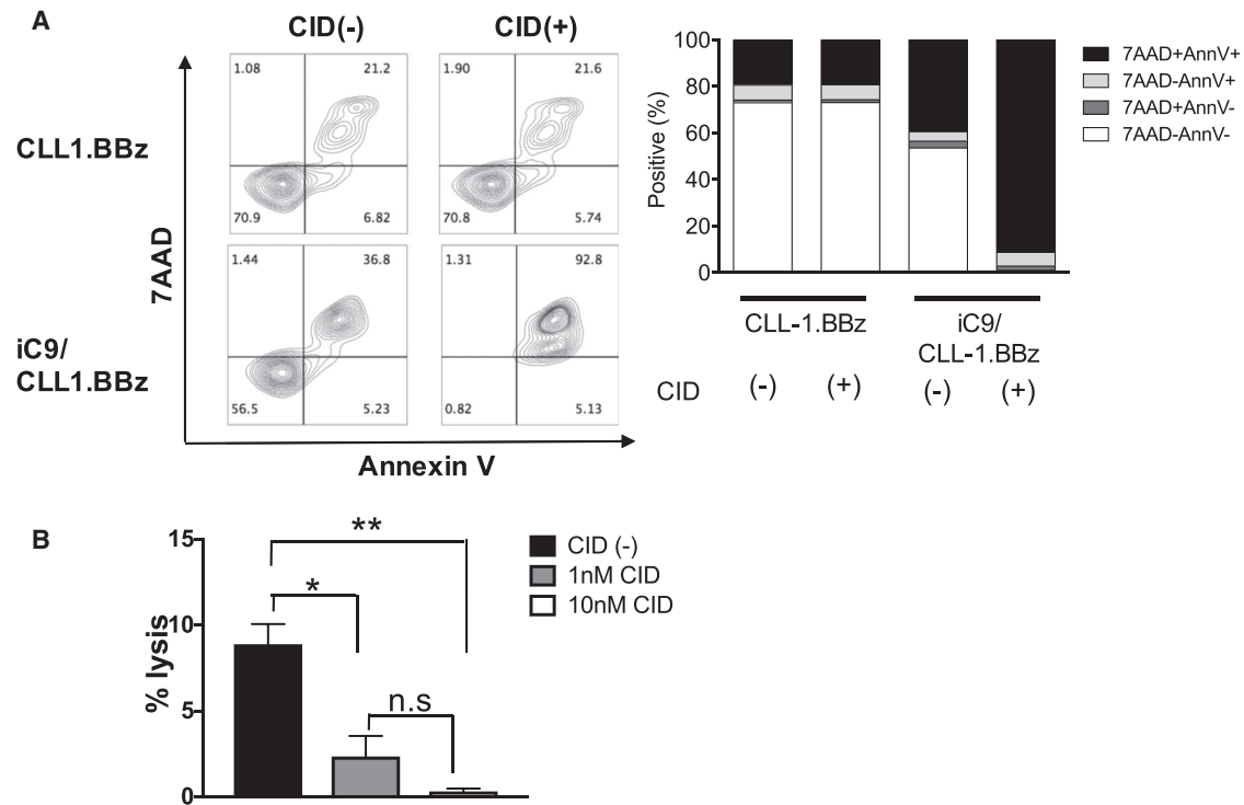
Figure 6. CLL-1.BB \zeta CAR-Ts Expressing an Inducible Caspase-9 Gene Are Eliminated by a Chemical Inducer of Dimerization
