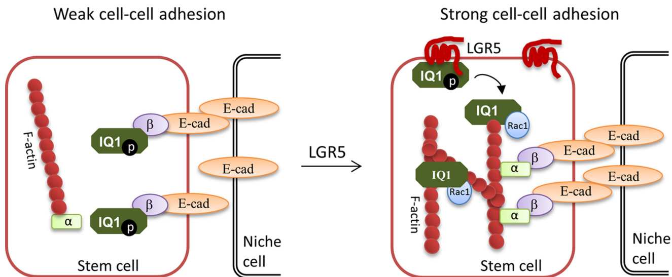
Figure 9. A schematic diagram illustrating the mechanism of LGR5 in the regulation of cell–cell adhesion through the IQGAP1–Rac1 pathway. In the absence of LGR5 ( left panel ), phosphorylated IQGAP1 (IQ1) is free of Rac1-GTP and can thus bind to \beta -catenin ( \beta ) to disrupt the interaction of \beta -catenin and \alpha -catenin ( \alpha ), leading to separation of the E-cadherin (E-cad) adhesion complex from the actin cytoskeleton and weak cell–cell adhesion. In the presence of LGR5 ( right panel ), the receptor reduces phosphorylation of IQGAP1, which then binds Rac1-GTP, leading to loss of binding to \beta -catenin as well as enhanced cross-linking of F-actin. This results in the linkage of E-cadherin adhesion complex to the cytoskeleton and stronger cell–cell adhesion.
