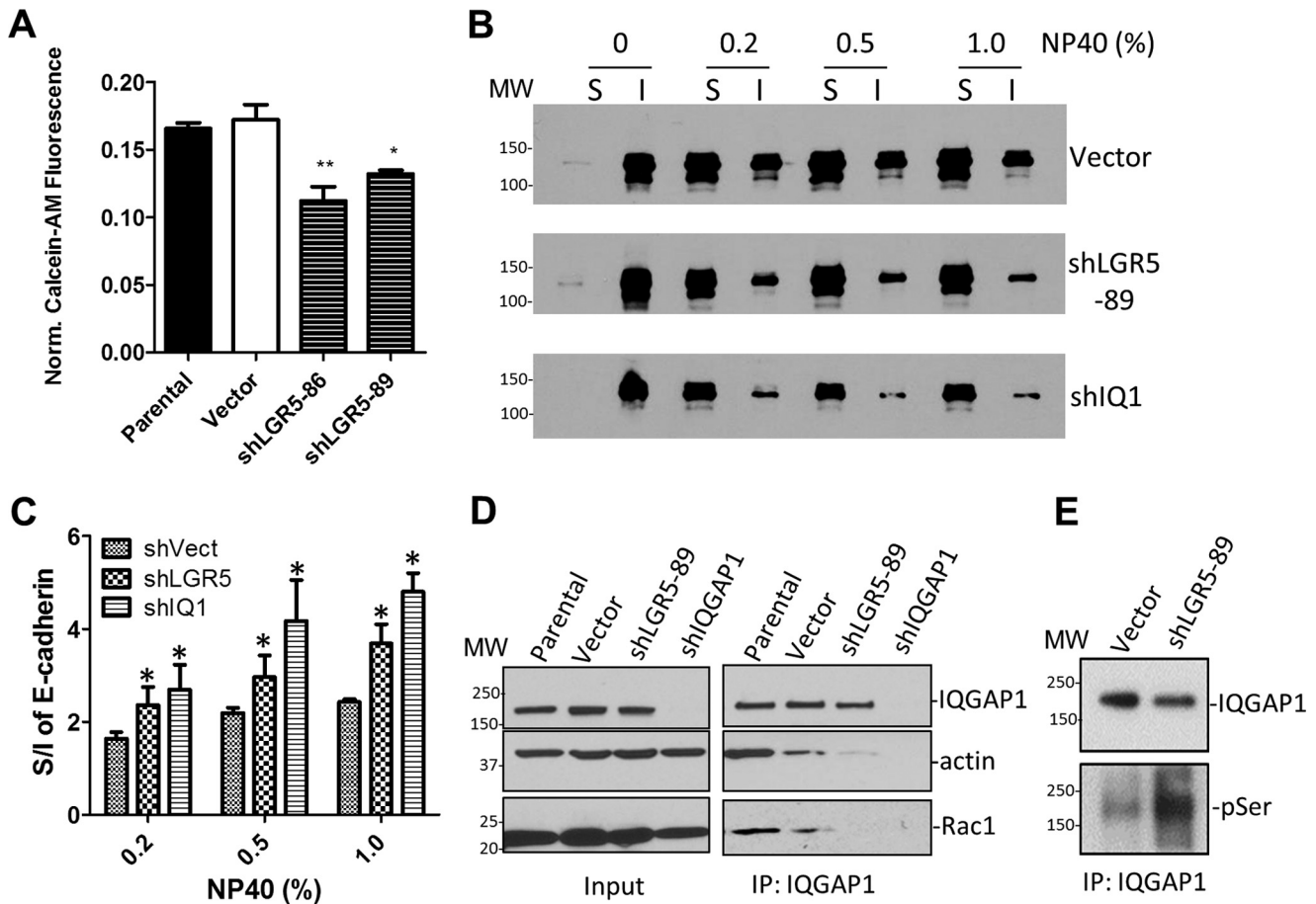
Figure 8. KD of LGR5 in LoVo cells resulted in loss of IQGAP1 interaction with Rac1/actin and decreased cell–cell adhesion. A , results of calcein-AM cell–cell adhesion assay. Error bars are S.E. ( n = 3 ). *, p < 0.05 and **, p \leq 0.01 versus controls. B , representative WB analysis results of soluble (S) and insoluble (I) E-cadherin in LoVo cells with vector control, KD of LGR5 (shLGR5-89), or KD of IQGAP1 (shIQ1) when extracted with the indicated concentrations of Nonidet P-40 (NP40). C , quantification of WB results of E-cadherin. Error bars are S.E. ( n = 3 ). *, p < 0.05 compared with vector cells. D , WB results of IQGAP1, actin, and Rac1 in control and LoVo cells with KD of LGR5 or IQGAP1. E , WB of serine phosphorylation of IQGAP1 in LGR5 KD LoVo cells.
