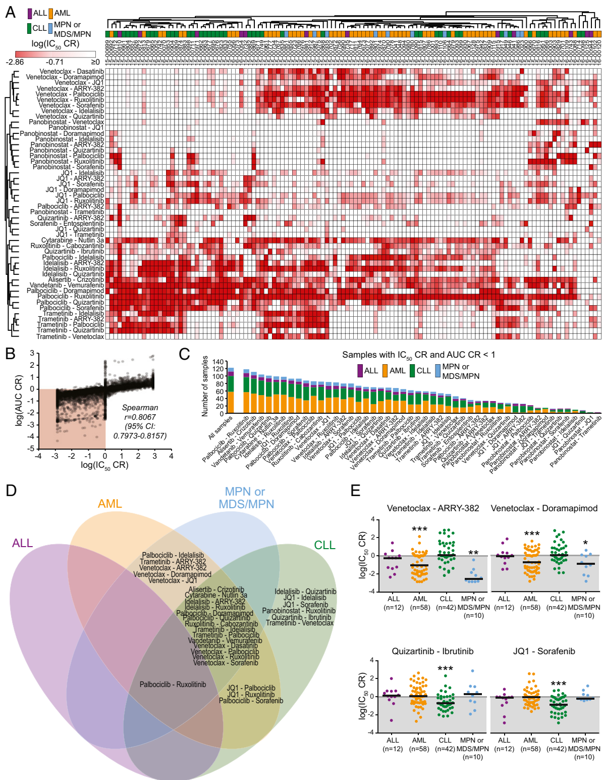
Fig. 1. Differential patterns of selective efficacy of small-molecule combinations relative to single agents. (A) Unsupervised hierarchical clustering of IC 50 CR values for 122 patients with leukemia across 48 tested combinations. IC 50 CR values were log-transformed and row- and column-clustered using Pearson correlation pairwise average linkage method. Darker red color (lower CR values) indicates drug combinations exhibiting higher efficacy than either single agent alone. Diagnostic category annotation of each sample is also shown. (B) Correlation of IC 50 CR and AUC CR effect measure values. Shaded region indicates sample/drug pairs for which the combination was more effective than either single agent (CR < 1) by both effect measures. (C) Distribution of effective drug combinations based on frequency and diagnostic category. Bar labeled “all samples” indicates diagnosis group breakdown for all 122 surveyed patient samples for comparison. (D) Overlap of significantly effective inhibitor combinations among four general diagnosis subgroups. Combinations for which median IC 50 CR and AUC CR were significantly <1 within each diagnostic subgroup are shown; combinations listed in overlapping regions were significantly effective in each subgroup. (E) Select examples of combinations by diagnostic subgroup. Scatter plots of log-transformed IC 50 CR values for select combinations. Black horizontal bars represent median CR. (*Median CR significantly <1 in that subgroup.)
