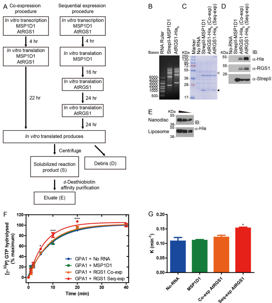
Figure 3. Synthesis of MSP1D1 and AtRGS1 from wheat germ cell-free extract (A) Schematic diagram for two procedures of cell-free synthesis and purification. Co-expression of MSP1D1 with AtRGS1 is compared to sequential expression (Seq-exp) of MSP1D1 followed by AtRGS1. (B) In vitro transcription RNA products for MSP1D1 and AtRGS1 were separated by 1.5% agarose gels. (C and D) Crude extract of in vitro translation for No-RNA negative control (No-RNA), MSP1D1 only (StrepII-MSP1D1), co-expressed AtRGS1 (Co-exp) and sequentially-expressed AtRGS1 (Seq-exp) were separated by 12% SDS-PAGE and detected by Coomassie Brilliant Blue Staining (C) , immunoblot analysis using anti- His 6 (D, upper) , anti-RGS1 (D, middle) and anti-StrepII (D, lower) antibodies. The open and closed arrowheads indicate the predicted molecular weights of AtRGS1 and MSP1D1, respectively. (E) Equal volume of crude AtRGS1 extracts in Nanodisc (sequential synthesis) and liposome were loaded in SDS-PAGE and immunoblotted by anti- His 6 antibody. The gradient indicates 2 fold dilution between lanes. (F) 250 nM of purified AtGPA1 was pre-incubated with [\gamma\text{-}^{32}\text{P}] GTP in ice cold buffer. Single turnover GTPase assays were initiated by the addition of GTP \gamma S containing buffer to
