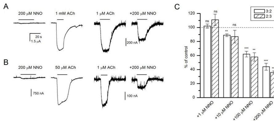
Figure 4. Direct activation and modulation of human \alpha 4\beta 2 receptors by trans -nicotine- N -oxide. (A) Sample traces from Xenopus oocytes expressing human \alpha 4\beta 2 nicotinic receptors in the stoichiometry of 3:2. Direct activation by 200 \mu\text{M} nicotine- N -oxide was minimal compared to the response to 1 mM ACh from the same cell. Co-application of 200 \mu\text{M} nicotine- N -oxide reduced the peak response to 1 \mu\text{M} ACh. (B) Sample traces from Xenopus oocytes expressing human \alpha 4\beta 2 nicotinic receptors in the stoichiometry of 2:3. Direct activating and modulating effects of nicotine- N -oxide are qualitatively similar to those observed in (A). (C) Concentration-response relationships for nicotine- N -oxide-mediated modulation of currents elicited by 1 \mu\text{M} ACh in oocytes expressing \alpha 4\beta 2 receptors in 3:2 or 2:3 stoichiometry. The data show the response ratio (peak amplitude in the presence vs. absence of nicotine- N -oxide) in %. All data points were collected from the same set of cells (5 for 3:2 and 4 for 2:3). Statistical analysis compares the response ratio to 100% (i.e., no effect) using a paired t-test. ns, not significant, **, P < 0.01 , ***, P < 0.001 .
