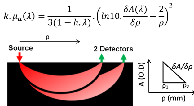
Fig. 2 Suzuki SRS concept illustrated
