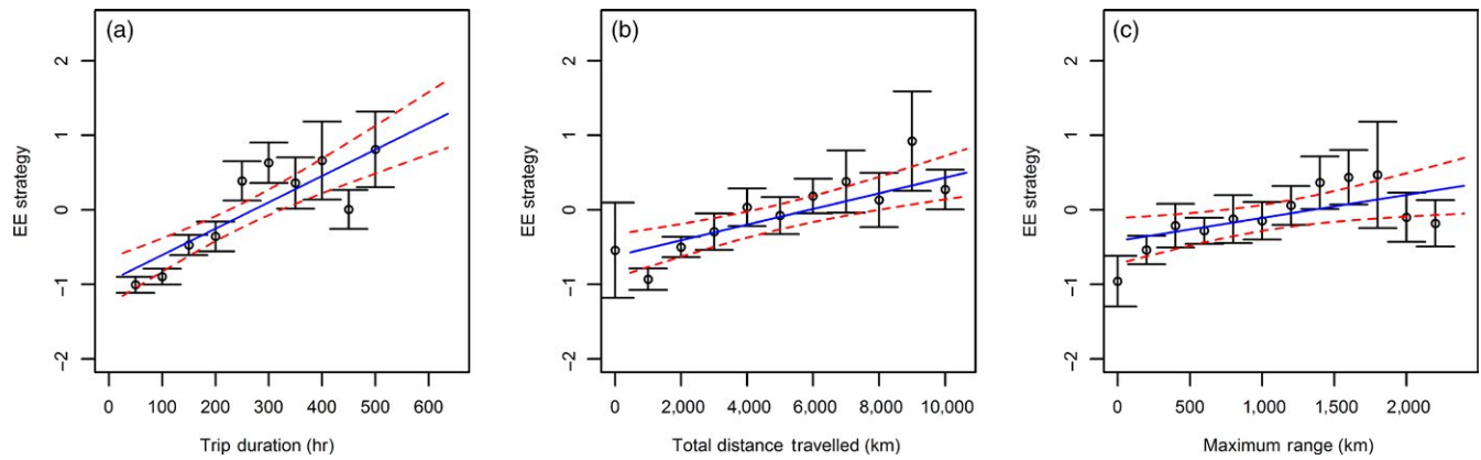
FIGURE 4 The relationship between EE strategy and foraging trip matrices. (a) Individuals which favour exploitation have longer foraging trip durations ( p < .001 ). N: [0, 50] (0), [50, 100] (11), [100, 150] (35), [150, 200] (28), [200, 250] (28), [250, 300] (31), [300, 350] (20), [350, 400] (15), [400, 450] (9), [450–840] (7), [500–840] (13). (b) Individuals which favour exploitation travel further during trips ( p < .001 ). N: [0,1000] (3), [1000, 2000] (21), [2000, 3000] (33), [3000, 4000] (24), [4000, 5000] (26), [5000, 6000] (19), [6000, 7000] (14), [7000, 8000] (15), [8000, 9000] (9), [9000, 10000] (12), [10000–17700] (21). (c) Individuals which favour exploitation have larger maximum ranges ( p < .001 ). N: [0, 200] (6), [200, 400] (31), [400, 600] (17), [600, 800] (24), [800, 1000] (15), [1000, 1200] (16), [1200, 1400] (18), [1400, 1600] (17), [1600, 1800] (23), [1800, 2000] (8), [2000, 2200] (11), [2200–3940] (11). Foraging metrics are grouped for plotting purposes. Raw data are shown in Appendix 2 Figure S2 [Colour figure can be viewed at wileyonlinelibrary.com ]
