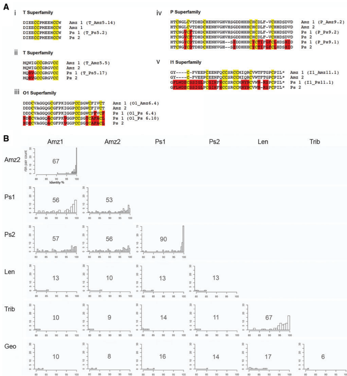
FIG. 5. —Inter- and intraspecific variation in Conus venom composition. (A) Sequence alignments of a selection of highly expressed conotoxins, where putative orthologs were identified in all four Turriconus specimens (predicted mature peptides and their names are shown); cysteines are highlighted in yellow and differences in amino acids are shown in red. *Predicted C-terminal amidation. (B) Histograms of rbh pair counts versus percent sequence identity for all species analyzed in this study. The total number of rbh pairs is depicted on graphs.
