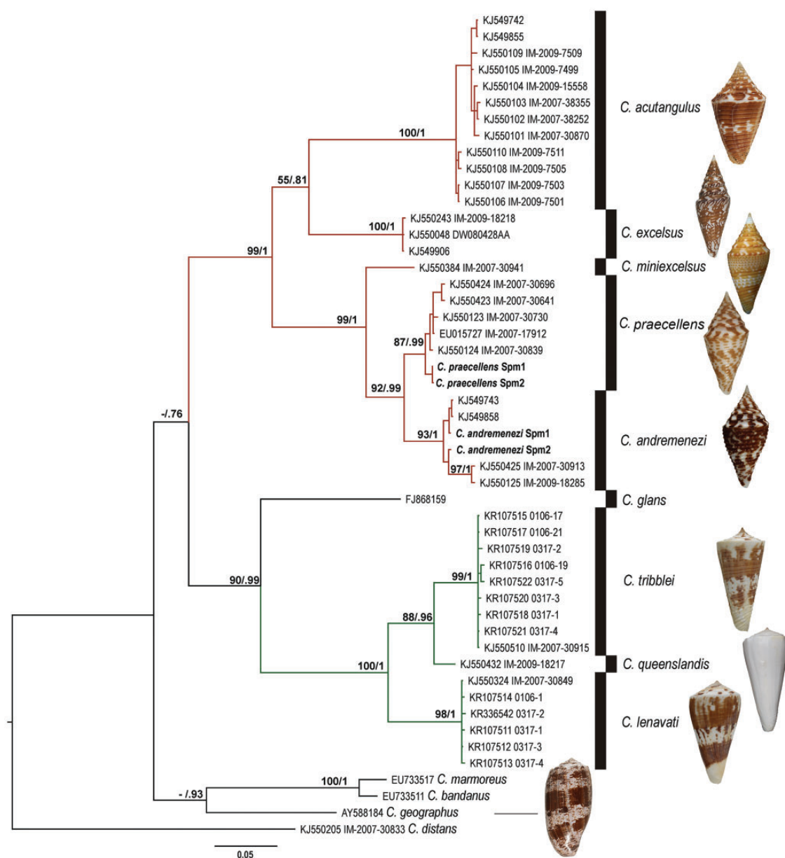
Fig. 2. —Bayesian phylogenetic tree of some Turriconus and Splinoconus species based on the analysis of the COI fragment. Support values at each node correspond to RaxML bootstrap (B)/Bayesian posterior probability (PP). The specimens for which venom gland transcriptomes were generated are labeled as C. andremenezi Spm1, C. andremenezi Spm2, C. praezellens Spm1, and C. praezellens Spm2. Shells of analyzed Turriconus and Splinoconus species and of C. geographus are shown right to the respective species clade.
