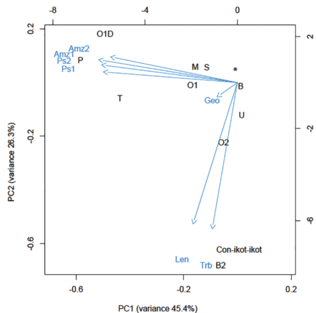
FIG. 4. —PCA of expression of individual superfamilies. Relative expression levels of conotoxin superfamilies were determined by mapping reads back to contigs with Bowtie2 (Langmead and Salzberg 2012). Expression levels were normalized to total read counts after trimming. Principal components were calculated using the prcomp package in R (R Core Team 2013). O1 \delta : \delta -like O1 superfamily; *Superfamilies that did not contribute to separation on PC1 and PC2.
