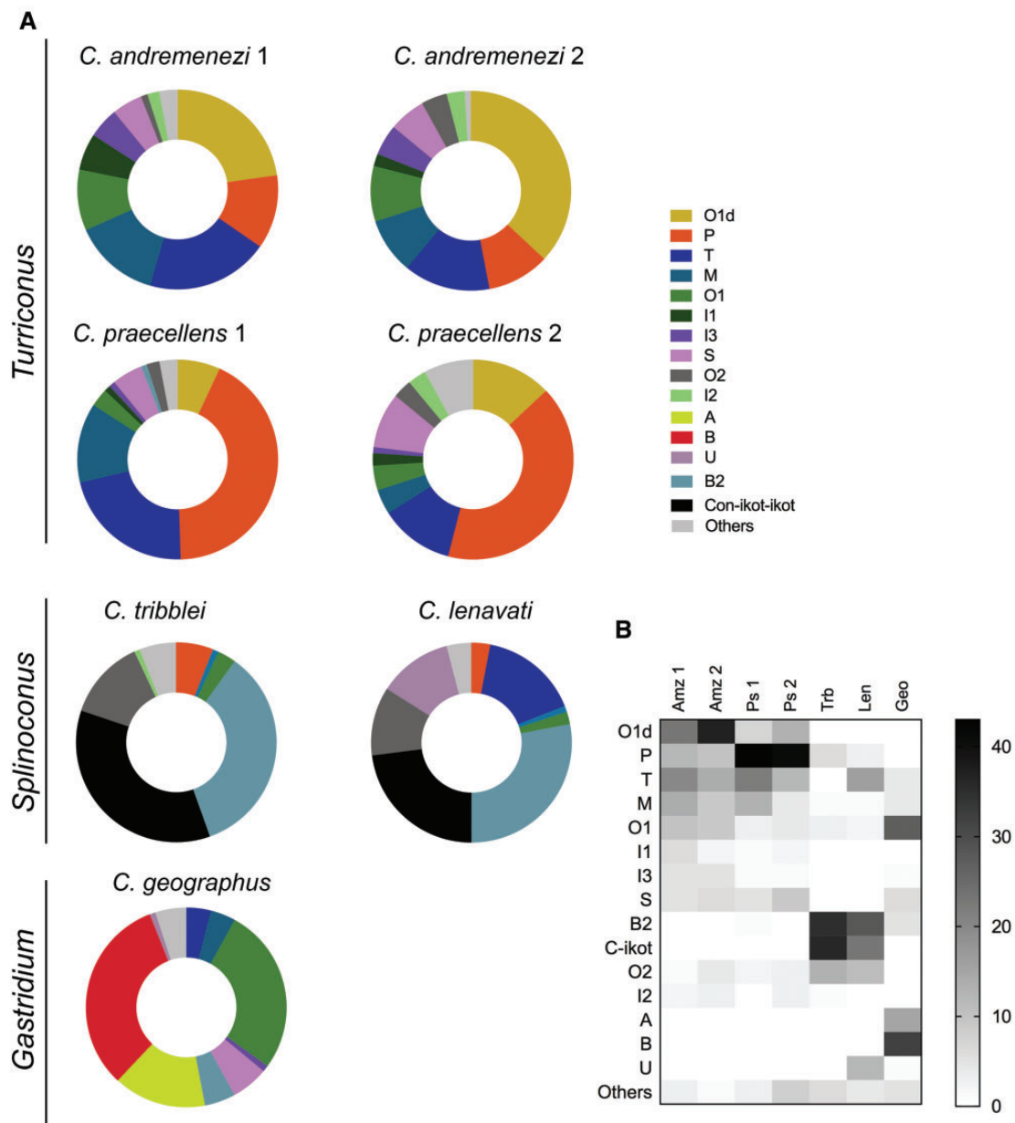
Fig. 3. —Comparison of relative toxin gene superfamily expression in C. andremenezi and C. praecellens with two members of the Splinoconus clades ( C. tribblei and C. lenavati ) and one member of the Gastridium clade ( C. geographus ). (A) Donut charts of expression levels. (B) Heat map showing a select number of superfamilies, including all that were highly expressed in the five species compared here. Plotted numbers represented normalized superfamily read counts. Amz1, C. andremenezi specimen 1; Amz2, C. andremenezi specimen 2; Ps1, C. praecellens specimen 1; Ps2, C. praecellens specimen 2; Trb, C. tribblei (pooled data from three individuals); Len, C. lenavati (pooled data from three individuals); Geo, C. geographus .
