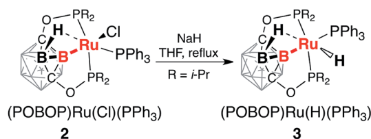
Scheme 2 Synthesis of (POBOP)Ru(H)(PPh 3 ) ( 3 ).
