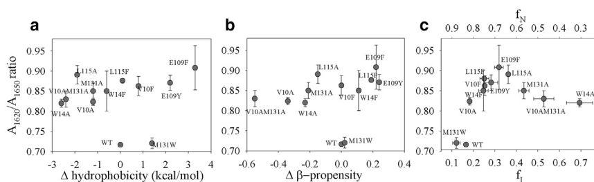
FIGURE 6 Dependence of the A_{1620}:A_{1650} ratio in IR spectra of WT sw ApoMb and its mutant forms on (a) changes in hydrophobicity, (b) changes in \beta -sheet propensity upon mutations, and (c) fractions of the I f_I and N states f_N at 40°C and pH 5.5.
