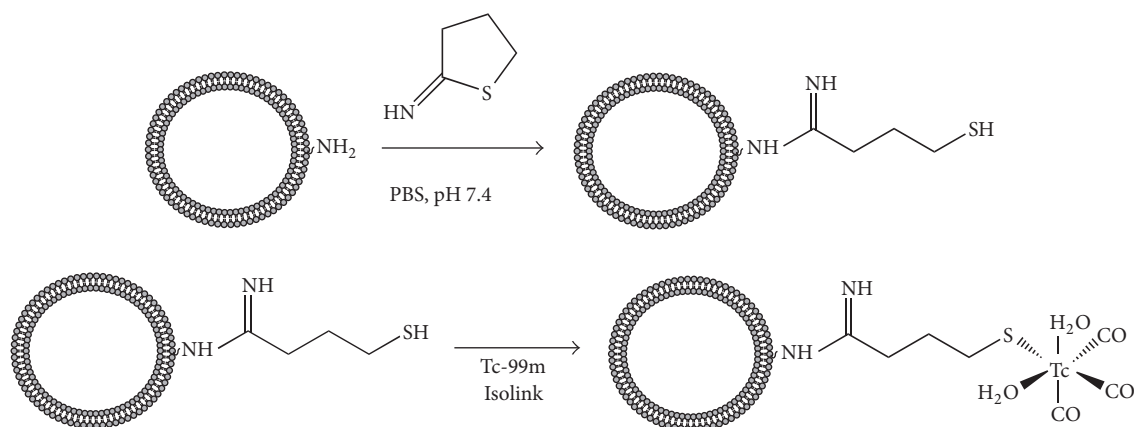
FIGURE 1: Surface modification of liposomes with 2-Iminothiolane (Traut's reagent) and labeling with ^{99m}\text{Tc} -tricarbonyl complex.
