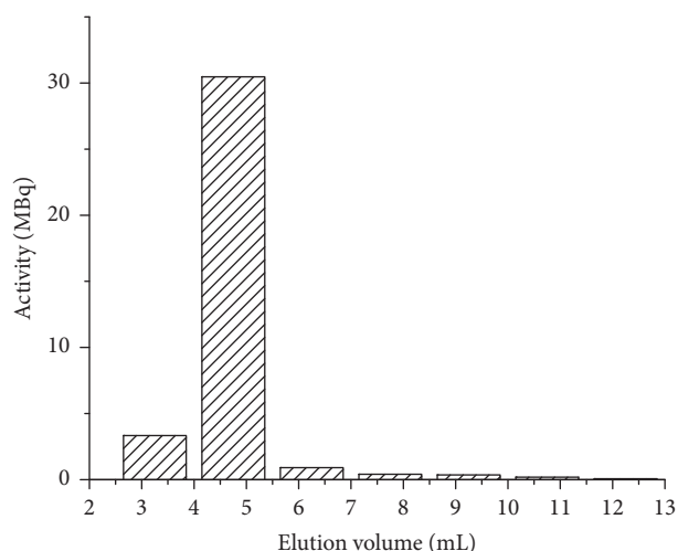
FIGURE 4: Elution profile of the 99m Tc-labeled liposomes on a PD-10 column. The first two fractions contain the labeled liposomes, while the free 99m Tc-tricarboonyl is eluted with the total volume of the column.
