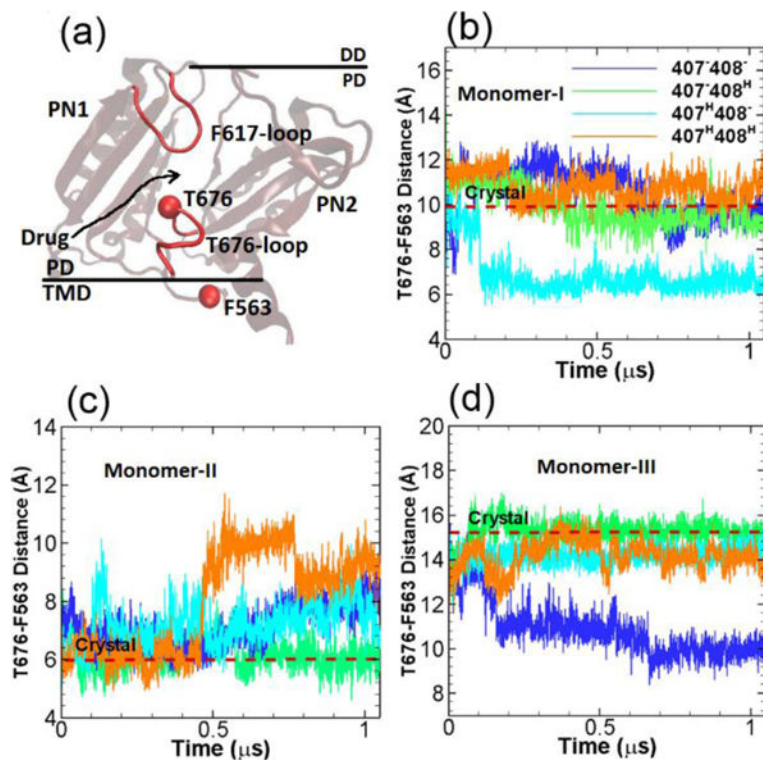
Figure 4. Cleft entrance. (a) Illustration of the relative locations of T676-loop, F617-loop in the porter domain and F563 in the TM domain. The time evolution of the T676-F563 distances in monomer I (b), monomer II (c) and monomer III (d) for the four model systems listed in Table 1. The values of T676-F563 distance in crystal structure (PDB ID: 2DHH) for the three monomers are indicated by red dashed lines for comparison. (Simulation results from the second realization can be found in Figure S2 from ESI.)
