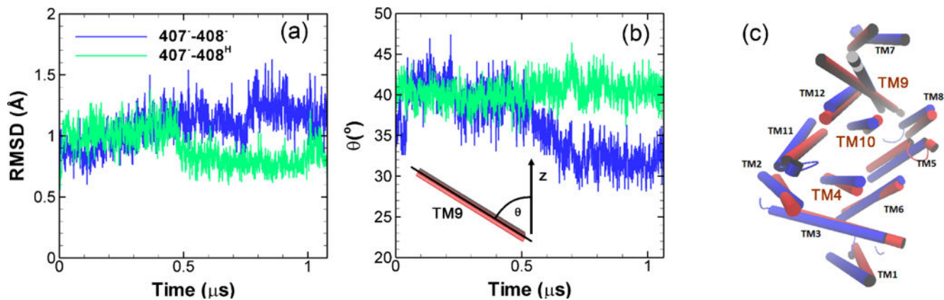
Figure 7. Structural changes in TM domain. (a) Time evolution of root-mean-square deviation (RMSD) relative to the crystal structure for TM10 (transmembrane \alpha -helix 10). (b) Time evolution of the angle ( \theta ) formed by TM9 and z-axis. (c) Cartoon representation of all 12 TM \alpha -helices in monomer III. Red: crystal structure of 2DHH. Blue: final structure from model system 1 (407 - -408 - ).
