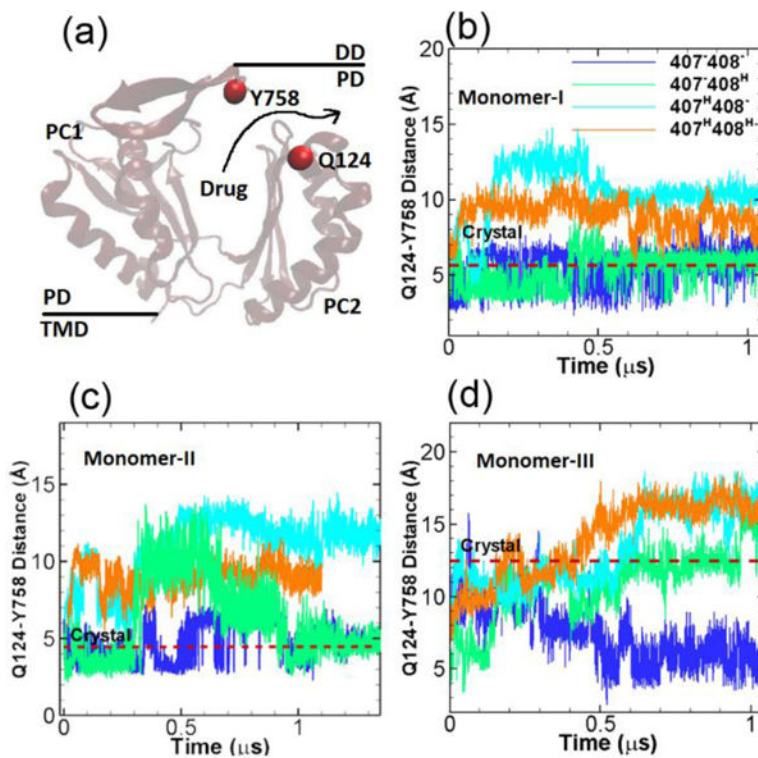
Figure 5. Exit channel. (a) Illustration of the relative locations of Y758 and Q124 at the exit channel. The time evolution of the Q124-Y758 distances in monomer I (b), monomer II (c) and monomer III (d) for the four model systems listed in Table 1. The values of Y758-Q124 distance in crystal structure (PDB ID: 2DHH) for the three monomers are indicated by red dashed lines for comparison. (Simulation results from the second realization can be found in Figure S3 from ESI.)
