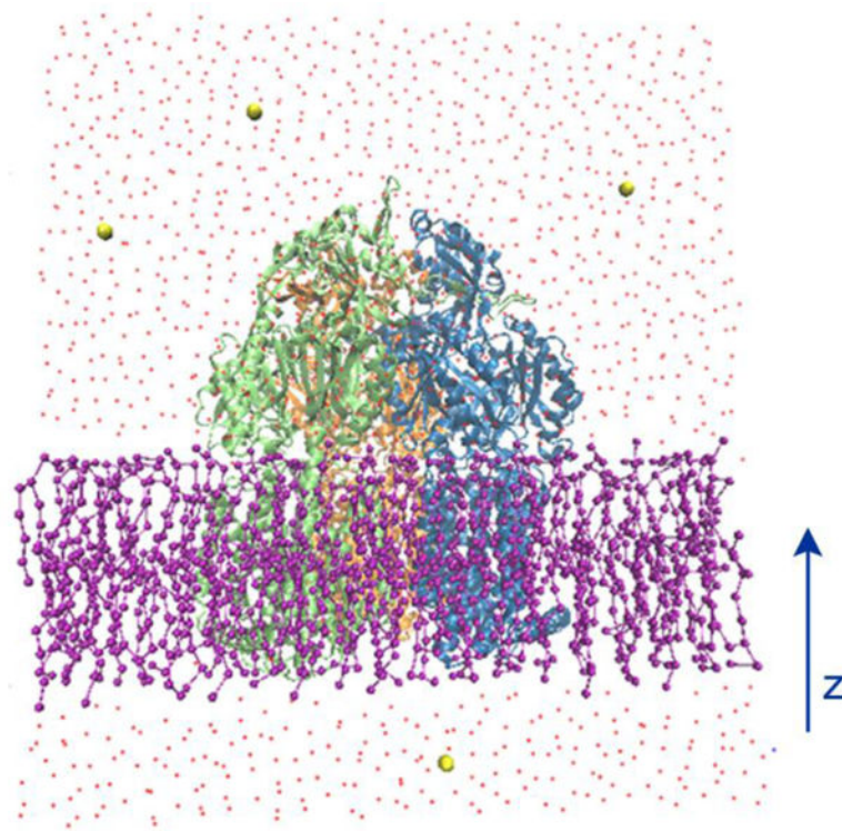
Figure 2. The illustration of the simulation system. AcrB protein (new cartoon representation) is embedded in a POPE lipid bilayer (ball and stick representation). Water molecules are represented by red dots and ions are shown with yellow sphere respectively.
