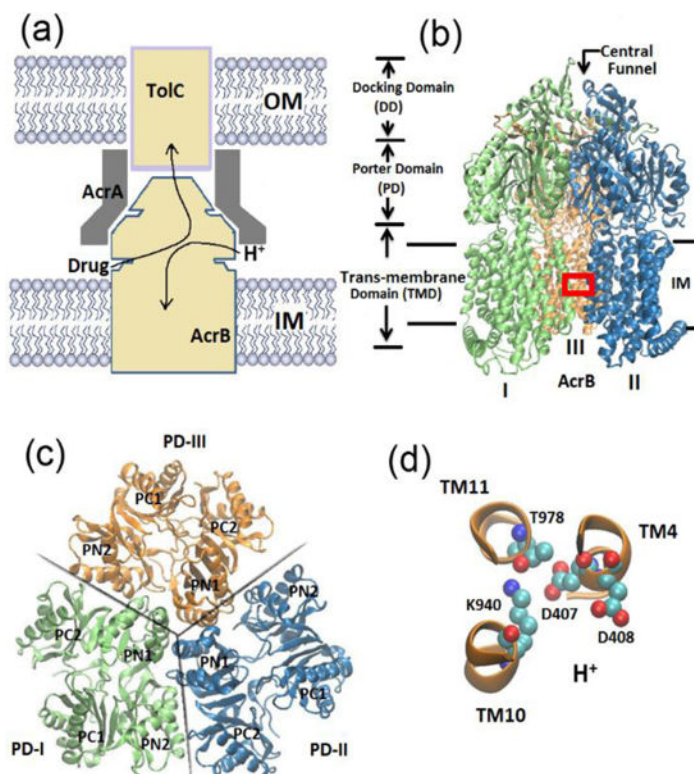
Figure 1. Multidrug resistance (MDR) system. (a) Schematic of the AcrB-AcrA-TolC tripartite efflux system. Arrows indicate the substrate/proton antiport directions. (b) New cartoon representation of the crystal structure of AcrB trimers. Each monomer can be decomposed into trans-membrane domain, porter domain and docking domain. (c) Top view of the porter domains. Each monomer is composed of four subdomains: PC1, PC2, PN1 and PN2. (d) Ball and stick representation of the key residues in TM domain (region indicated by red box in (b)): Asp 407, Asp 408, Lys 940 and Thr978.
