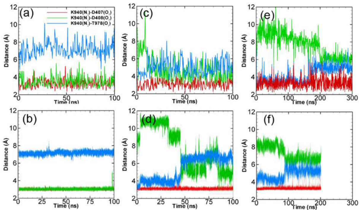
Figure 3. Side chain dynamics at the TM domain. The time evolution of K940-D407 (red), K940-D408 (green) and K940-T978 (blue) distances for monomer II (model 1) (a), monomer III (model 1) (c) and monomer III (model 2) (e). (b), (d) and (f) shows the corresponding results of all-atom simulations from Ref. 18 (Simulation results from the second realization can be found in Figure S1 from ESI.)
