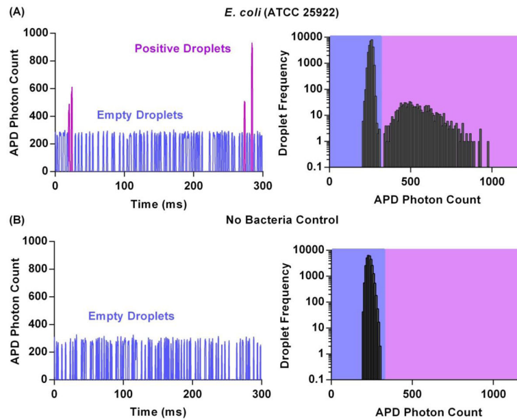
Fig. 2. Rapid bacterial growth quantification with E. coli (A) The fluorescence intensity of each droplet is quantified. Droplets containing growing bacteria (positive droplets) emit greater fluorescence than empty droplets. The data is further plotted in a histogram with bin size of \sim 10 for population distribution analysis. For an input concentration of 10^7 CFU/mL of E. coli , an average of 903 \pm 137 droplets out of 30000 total droplets comprise of the positive droplet population. Standard deviation is from triplicate experiments. (B) When no bacteria are input into the platform, no positive peaks are detected and only the negative population of background/empty droplets is present.
