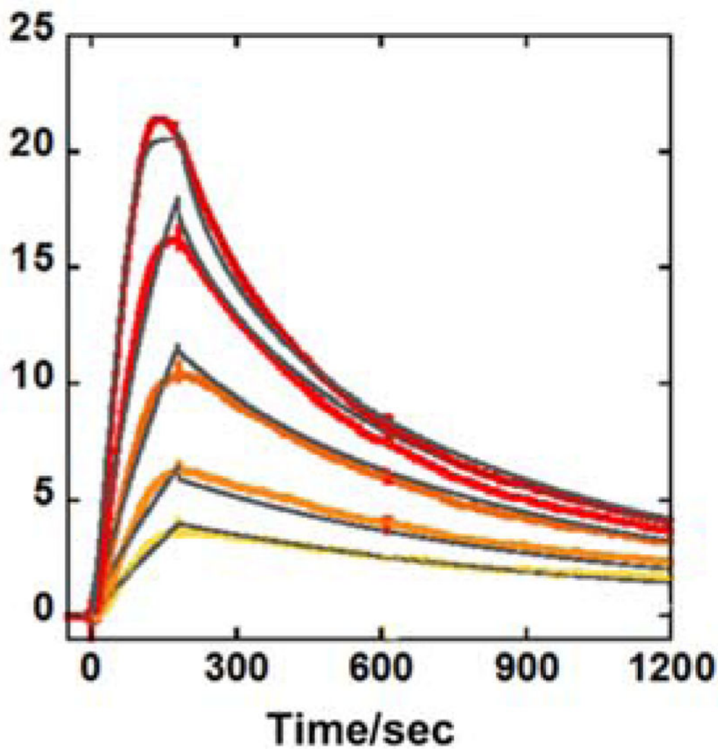
Fig. 2. Representative SPR sensorgrams for DB2528 in the presence of GAAAC DNA, concentrations of DB2528 from bottom to top are 10, 15, 30, 50, and 100 nM. The solid black lines are best-fit values for the global kinetic fitting of the results with a single site function.
