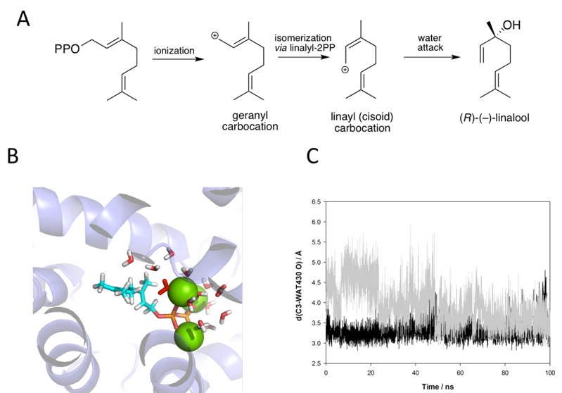
Figure 8. Mechanistic proposal for bLinS and MD of bLinS with GPP and three Mg 2+ ions. (A) Schematic outline representing the conversion of GPP to the linalool product by bLinS. (B) Active site of bLinS in the dominant cluster from MD simulations with GPP and three Mg 2+ ions. GPP is shown with cyan carbon atoms, bLinS is shown in purple in cartoon form and the Mg 2+ ions are shown as green spheres. Water molecules within 5 Å of GPP are shown in stick form, with the water molecule closest to C3 of GPP shown in red. (C) The distance between C3 and O of WAT430 over the course of two 100 ns MD simulations.
