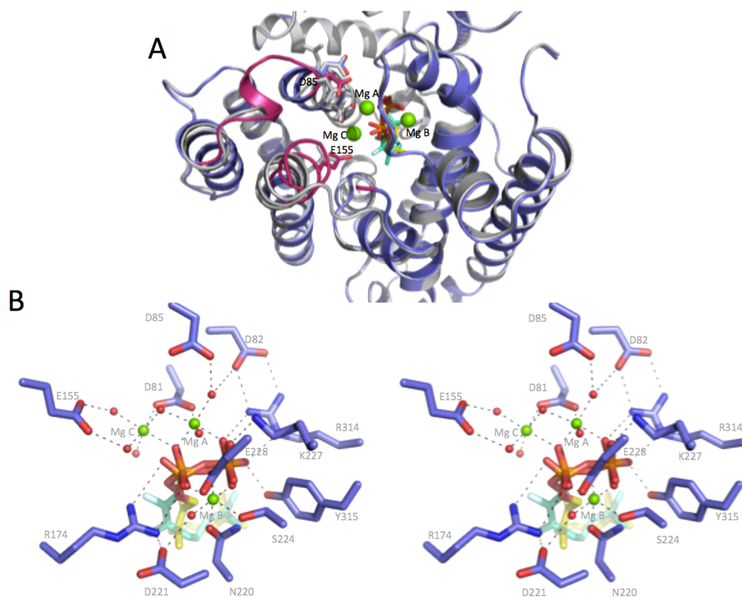
Figure 4. Structure of bCinS in complex with FGPP. (A) Cartoon representation of an overlay of the bCinS-FNPP complex structure (in gray) with the bCinS-FGPP/FNPP structure obtained by soaking bCinS-FNPP with GFPP (in blue). A loop region C-terminal to D85 as well as the region surrounding E155 adopt distinct conformations in response to binding of \text{Mg}^{2+} C, these regions are colored in red. (B) Stereoview of the FGPP/FNPP- \text{Mg}^{2+} ion binding site. Key polar interactions are shown by dotted lines.
