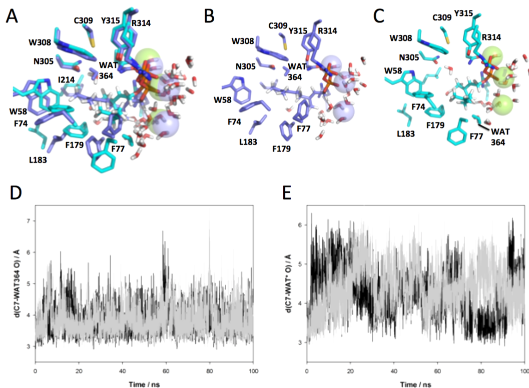
Figure 6. MD of bCinS with three Mg^{2+} ions and GPP or NPP. (A) Active site of bCinS in the dominant cluster from MD simulations with of bCinS/GPP (purple) and bCinS/NPP (cyan). Water molecules within 5 Å of GPP are shown in stick form and the closest water molecule to C7, the site of attack by the water molecule, is colored in purple for bCinS/GPP and cyan for bCinS/NPP. (B) and (C) show the same view of bCinS/GPP and bCinS/NPP alone, respectively. (D) The distance between C7 and O of WAT364 over the course of two 100 ns MD simulations of bCinS/GPP. (E) The distance between C7 and O of the closest water molecule to C7 of NPP over the course of two 100 ns MD simulations.
