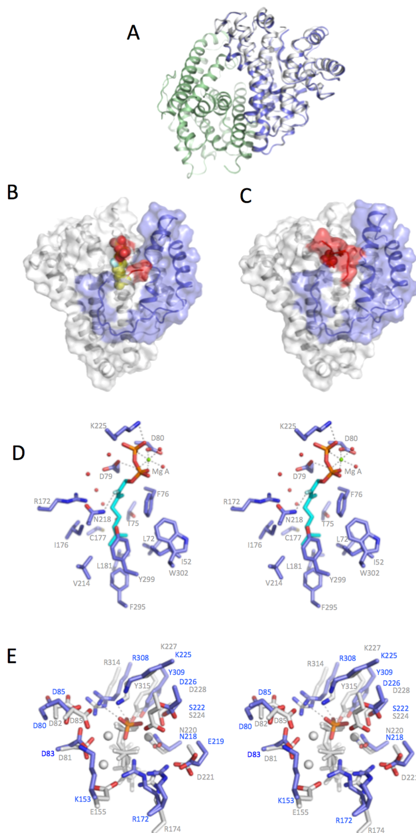
Figure 7. Structure of bLinS in apo and FGPP complex form. (A) Cartoon representation of the apo bLinS dimer, with one monomer colored in green and the second monomer in blue. The latter is overlaid with the first monomer (in gray) revealing small changes in conformation distant from the dimer interface. (B) Cartoon representation of monomer A bound to FGPP. The N-terminal region is shown in blue and the (here disordered) C-terminal region in red. (C) Cartoon representation of the monomer B bound to phosphate. Orientation and color coding are as in panel B. The ordering of the C-terminus and the partial closing of the N-terminal regions occludes the phosphate from solvent, in contrast to the solvent exposed nature of the diphosphate group in monomer A. (D) Stereoview of the active site of bLinS monomer A in complex with FGPP. Key polar interactions are shown by black dotted lines. (E) Stereoview of the active site of bLinS monomer B (in blue) in overlay with the active site of bCinS in complex with FGPP/FNPP (in gray).
