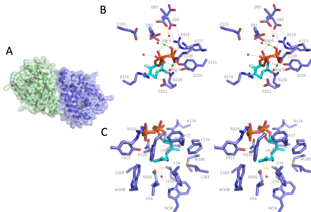
Figure 2. Structure of bCinS in complex with FNPP. (A) Cartoon representation of the bCinS dimer with the solvent accessible surface shown color coded per monomer. (B) Stereoview of the FNPP-Mg 2+ ion binding site. Key polar interactions are shown by dotted lines. The electron density indicates multiple positions of the diphosphate moiety as well as several Mg 2+ binding residues. (C) Stereoview of the FNPP hydrophobic binding pocket. A single water molecule is present, located close to the C6 atom.
