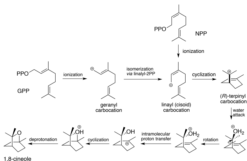
Figure 5. Mechanistic proposal for bCinS. A schematic outline of a putative mechanism for the conversion of GPP and NPP to the 1,8 cineole product by bCinS. Taking into account the observed position and orientation of the bCinS ligands and adjacent water molecules, we propose that the ( R )-terpinyl carbocation intermediate is formed, followed by the anti -addition of water, requiring a rotation step prior to heterocyclization.
