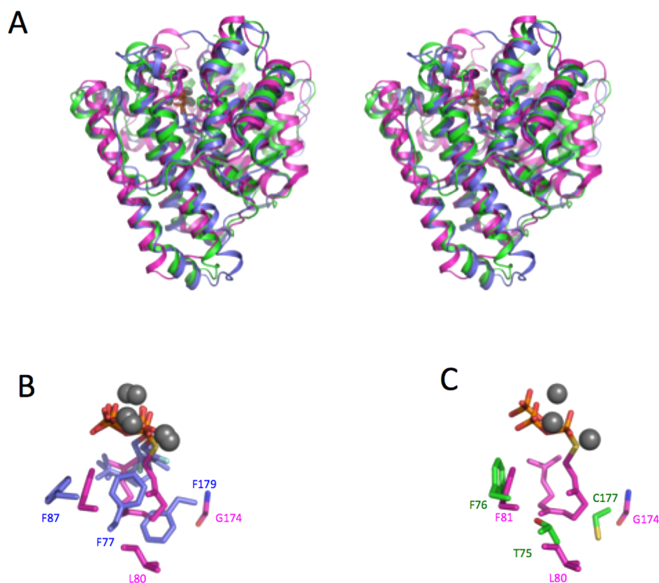
Figure 9. bLinS and bCinS are related to bacterial sesquiterpene synthases. (A) Stereoview of a cartoon representation of a structural overlay of bLinS (monomer B; in green), bCinS FGPP/FNPP (in blue) and aristolochene synthase (ATAS) (PDB code 4KUX) in complex with a C15 substrate analogue (in magenta). (B) Active site overlay of bCinS and ATAS, color coding as in panel A. (C) Active site overlay of bLinS (monomer B) and ATAS, color coding as in panel A.
