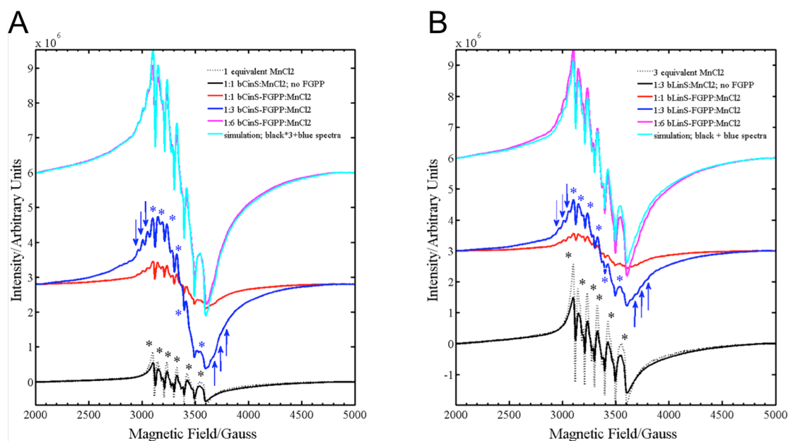
Figure 3. EPR confirms binding of 3 \text{Mn}^{2+} in solution. cw-EPR spectra of ' \text{Mn}^{2+} ' substituted bCinS (A) and bLinS (B) protein samples with varying equivalents of \text{Mn}^{2+} concentration with or without FGPP measured as a frozen solution along with standard \text{MnCl}_2 . The plot shows the multiplet EPR signal arise from the \text{Mn}^{2+} ion around the g = 2 region (from 250 to 400 mT).
