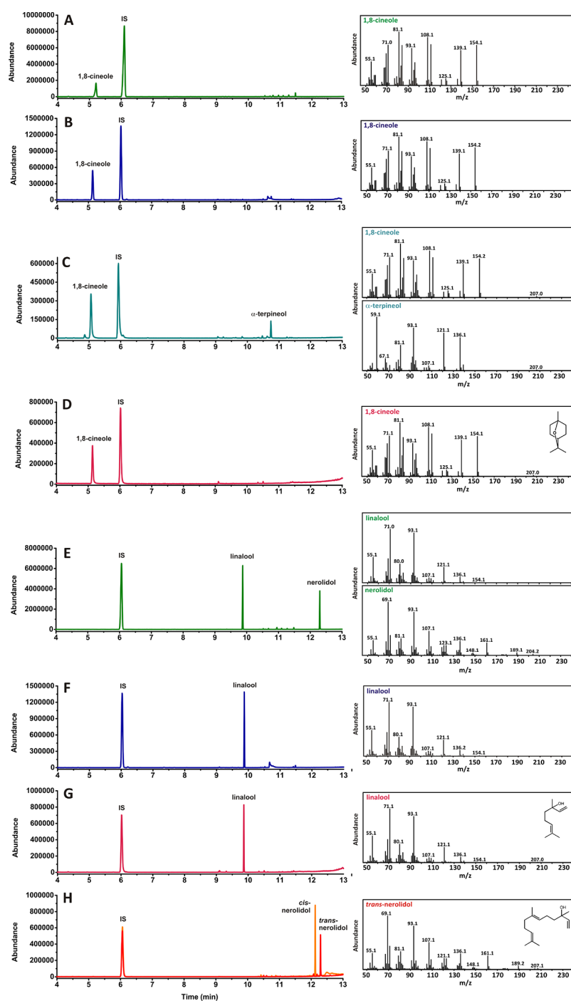
Figure 1. GC-MS analysis of bCinS and bLinS. (A) bCinS product profile when inserted in an engineered E. coli strain capable of overproducing GPP. (B) bCinS conversion of GPP (2 mM) in vitro . (C) bCinS conversion of NPP (2 mM) in vitro . (D) 1,8-cineole standard (0.1 mg/mL). (E) bLinS product profile when inserted in an engineered E. coli strain capable of overproducing GPP. (F) bLinS conversion of GPP (2 mM) in vitro . (G) R -(–)-linalool standard (0.1 mg/mL). (H) cis - and trans -nerolidol standards (0.1 mg/mL). IS = internal standard ( sec -butyl benzene).
