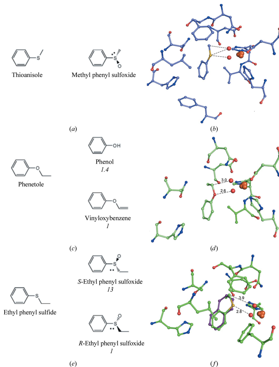
Figure 3 Products formed by NDO with thioanisole ( a ), phenetole ( c ) and ethylphenylsulfide ( e ). Approximate ratios of products detected in biotransformation assays are shown in italics below the products. Wild-type NDO in complex with phenetole ( d ), with ethylphenylsulfide ( e ) overlapped with that with naphthalene ( f ) and with thioanisole ( b ), with active-site residues of NDO represented by sticks with green C atoms. The mononuclear iron (large orange sphere) and modeled dioxygen from PDB entry 1o7n (small red spheres) are also shown.
