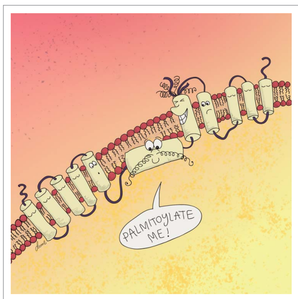
Figure 1. An amphipathic \alpha -helix directs palmitoylation of NCX1. Palmitoylation of NCX1 at C739 requires an \alpha -helix at the C-terminal end of the NCX1 regulatory intracellular loop. The hydrophobic face of the helix probably interacts with the membrane, while the cytosolic hydrophilic face is likely recognized by the cellular palmitoylation machinery.
