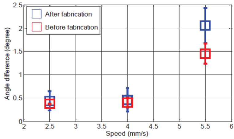
Fig. 7. Mean value of the angle difference with respect to the insertion speed and stylet condition (before and after fabrication). Each trial was repeated five times.
