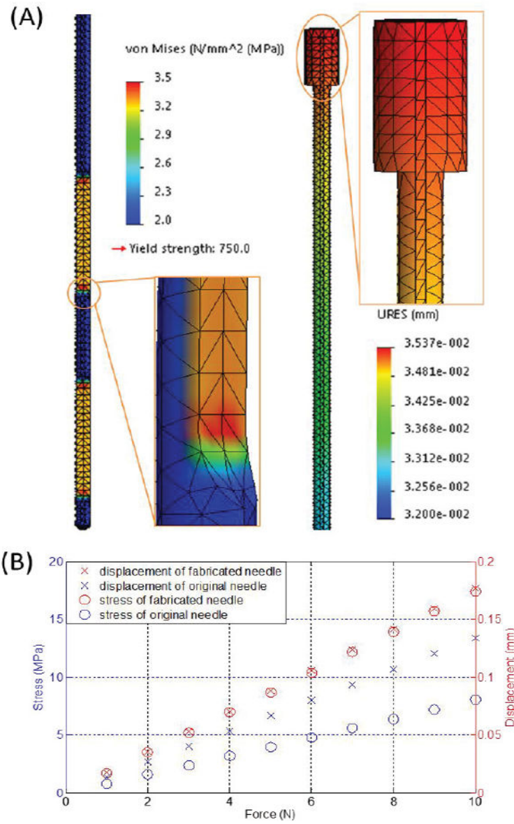
Fig. 5. (A) Case study of the stylet maximum stress (left) and displacement (right) at an applied insertion force of 2N; (B) Stress and displacement with respect to insertion forces ranging from 1N to 10N.
