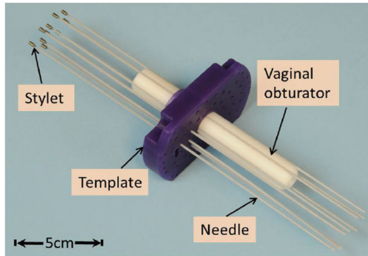
Fig. 1. Applicators for MR-guided gynecologic brachytherapy. The dimensions of the template are 10.7 \times 7 (L \times W) \text{cm}^2 with thickness of 1.5cm; the obturator is: 15-cm long with diameter of \text{\O}2.2\text{cm} .
