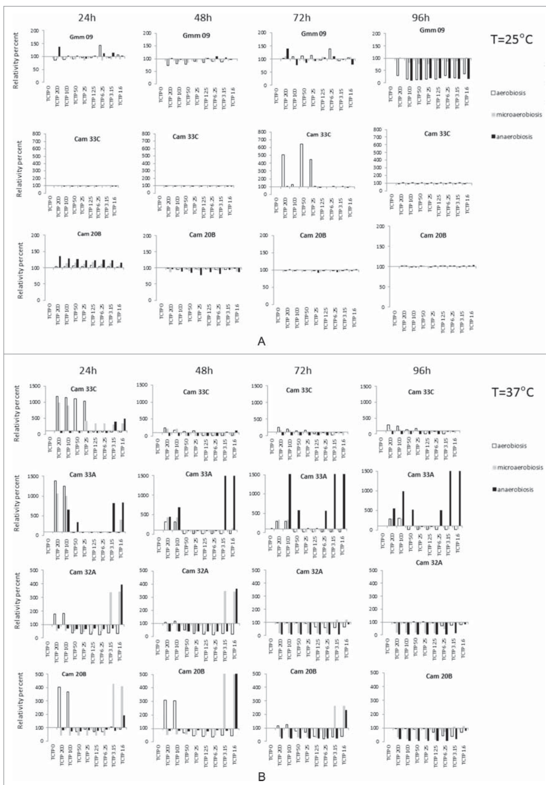
Figure 6. Effect of different concentrations of rTbgTCTP on bacteria growth. The effect was tested at 25^{\circ}\text{C} (A) and 37^{\circ}\text{C} (B-E), under 3 different atmosphere compositions: aerobiosis (white column), microaerobiosis (gray column), and anaerobiosis (black column). Histograms compare, for a given experimental condition (and for each time), the OD of the tested culture (with TCTP at a given concentration) with the OD of the corresponding control culture without TCTP (assigned to the value 100%). The results are the mean of triplicate experiments.
