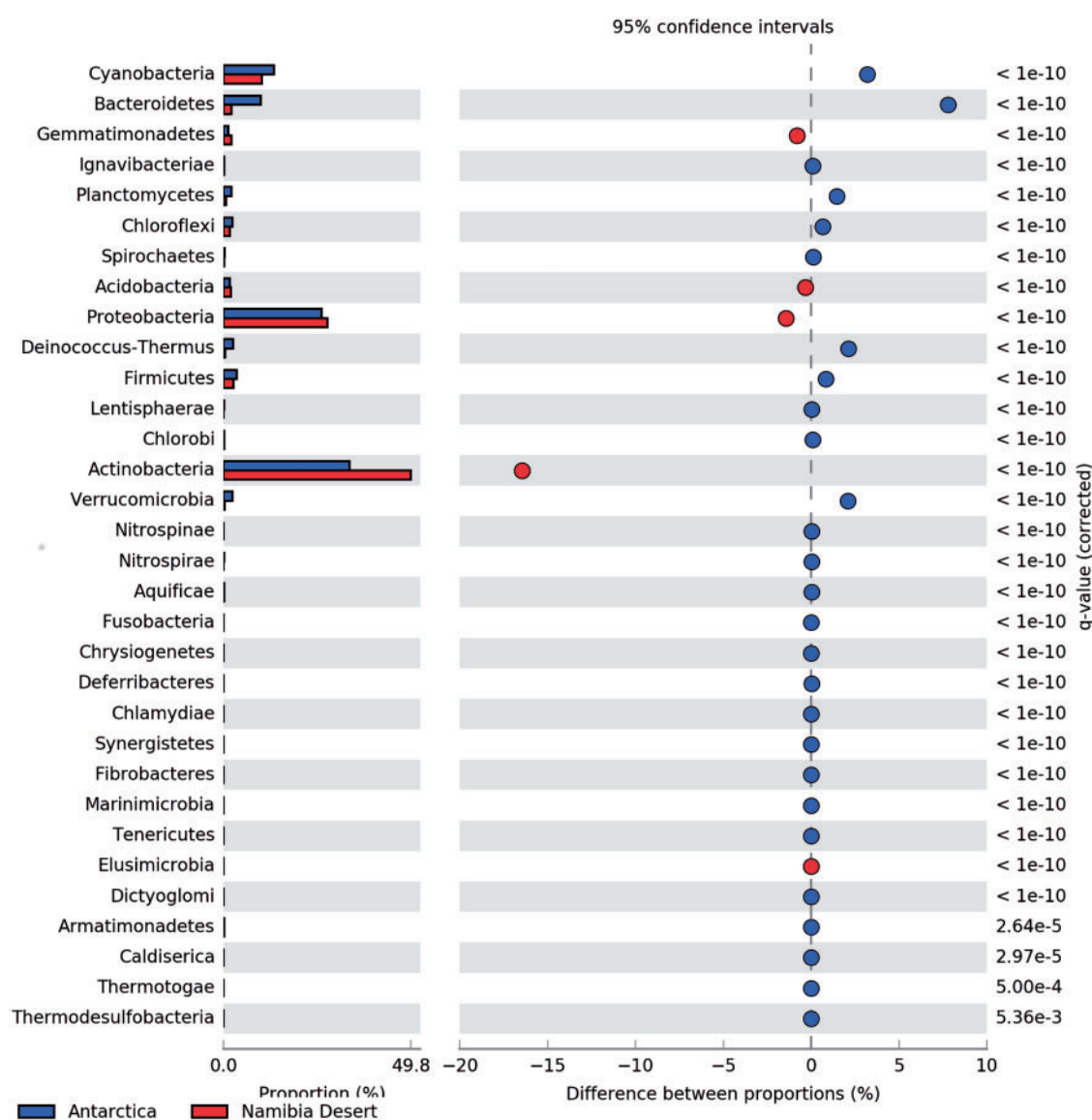
Fig. 1. —Statistical analysis of taxonomic profiles (at phylum level) of Antarctic and the Namib Desert metagenomes by BlastX of contigs against Non Redundant NCBI database. Phyla, which were in high relative abundance, have significant indicators.
