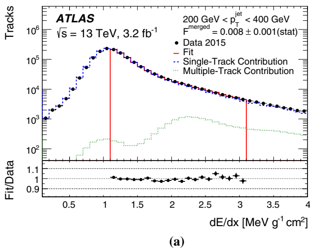
Fig. 16 Data dE/dx measurement distributions (black circles) with fit results (solid line) are shown for a 200 \text{ GeV} < p_T^{\text{jet}} < 400 \text{ GeV} and b 1000 \text{ GeV} < p_T^{\text{jet}} < 1200 \text{ GeV} . The single-track template scaled by
