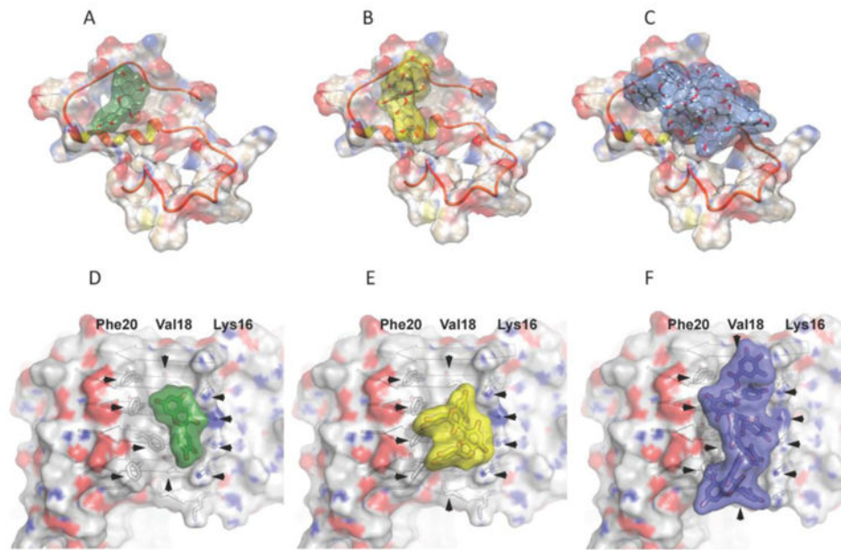
Fig. 8. Models of complexes between A \beta 40 and GSPE monomers, dimers or oligomers Panels are: (A) docked monomer, (B) docked dimer, and (C) docked oligomer. The peptide backbone is illustrated as in orange and red. Panels D-F show the monomer (D), dimer (E), and oligomer (F) interacting with backbone atoms of an A \beta fibril. Fibril side-chains are shown in grey and extend from \beta -strands oriented equatorially relative to the fibril axis. Hydroxyl groups form hydrogen bonds to Lys16 of A \beta . Apolar interactions may occur among the aromatic rings of GSPE and the hydrophobic patches formed by Val18 and Phe20 of A \beta .
