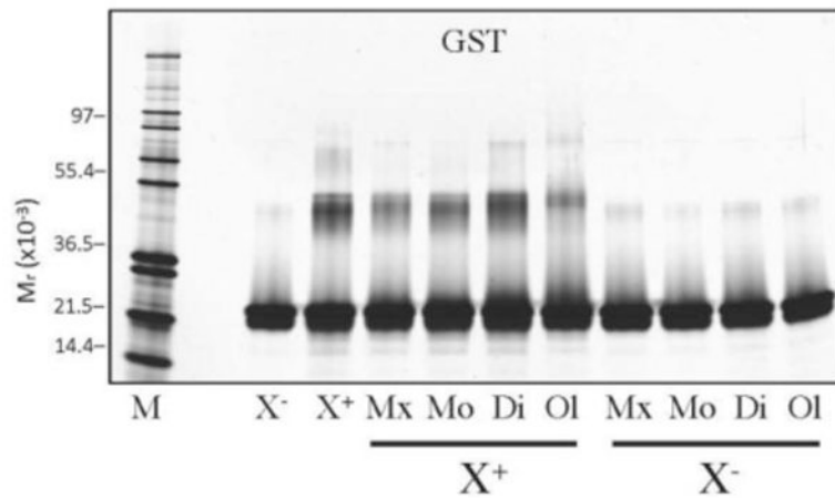
Fig. 2. Oligomerization of A \beta in the presence of GSPE
