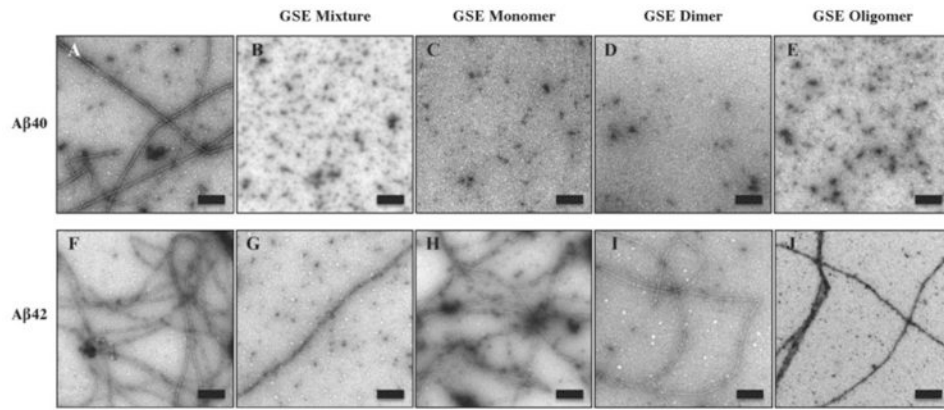
Fig. 6. Electron microscopy of Aβ40 and Aβ42 with and without equimolar GSPE mixture, oligomer, dimer, or monomer
