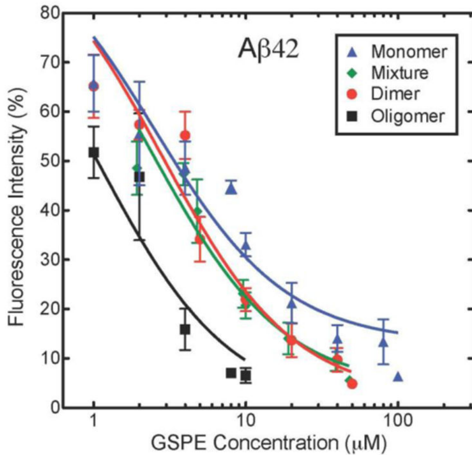
Fig. 5. Concentration-dependence of inhibition of Aβ ThT fluorescence by GSPE (A) Aβ40 and (B) Aβ42 were incubated with varying concentrations of GSPE mixture, oligomer, dimer, or monomer. Final ThT fluorescence intensities were measured for each sample and normalized to the corresponding Aβ40 or Aβ42 alone. The data herein were used to derive IC_{50} values (Table 3).
