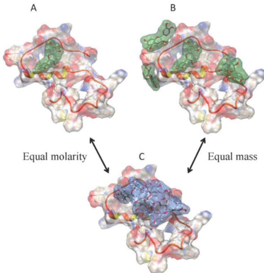
Fig. 7. GSPE:Aβ interactions
