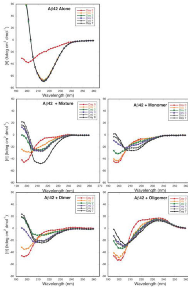
Fig. 3. Effect of GSPE on the evolution of Aβ secondary structure
