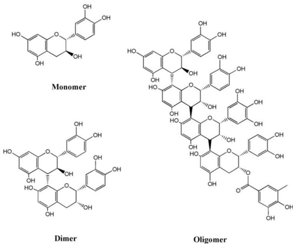
Fig. 1. Structures of representative GSPE components
