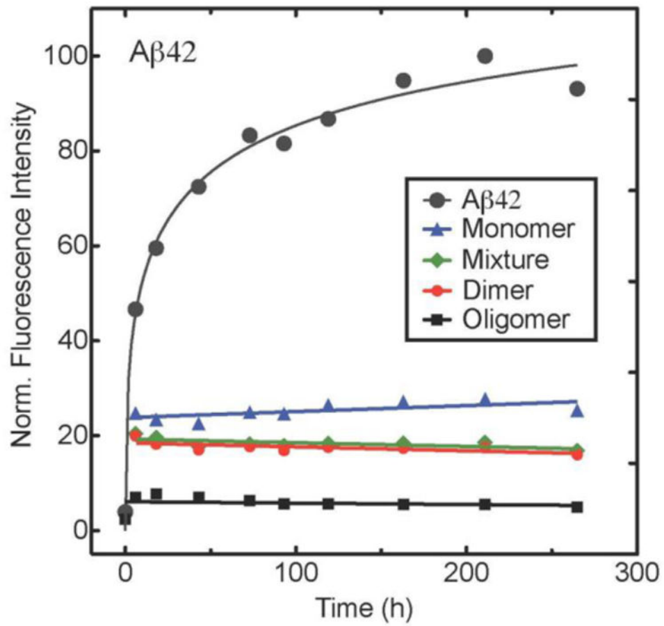
Fig. 4. Effect of GSPE fractions on the evolution of ThT fluorescence from A \beta ThT fluorescence intensities were measured for (A) A \beta 40 and (B) A \beta 42 incubated alone, or with, GSPE fractions. Fluorescence intensities were normalized to the highest value for each experimental condition. Data shown are representative of each of 4 replicates for A \beta 40 and 5 replicates for A \beta 42.
