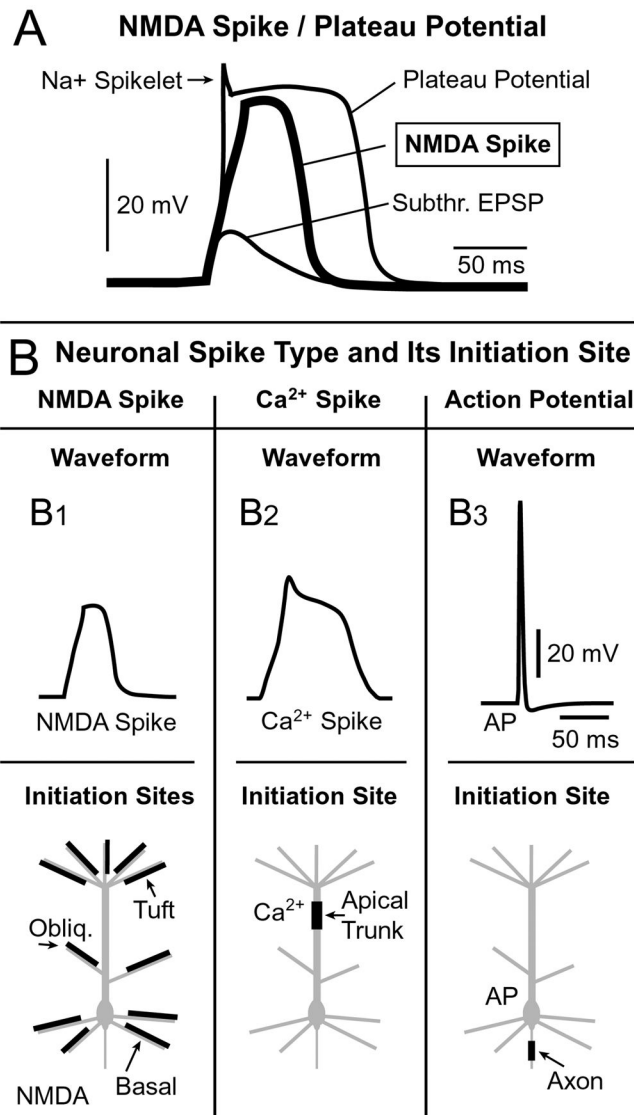
Figure 1. Each Class of Neurites (Basal, Oblique, Tuft, Apical Trunk, and Axon) Supports a Characteristic Regenerative Potential (Spike)
