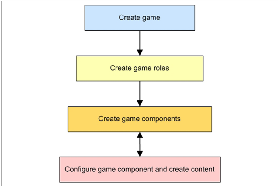
Figure 2. Authoring process.
