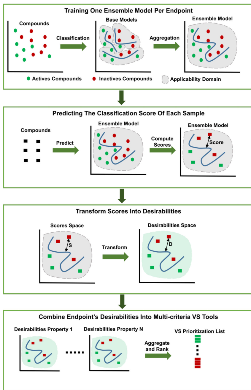
Figure 2. Overall workflow of the proposed methodology.
