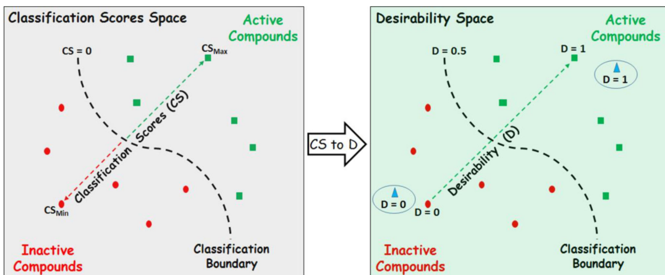
Figure 3. Transforming classification scores into desirability values.
