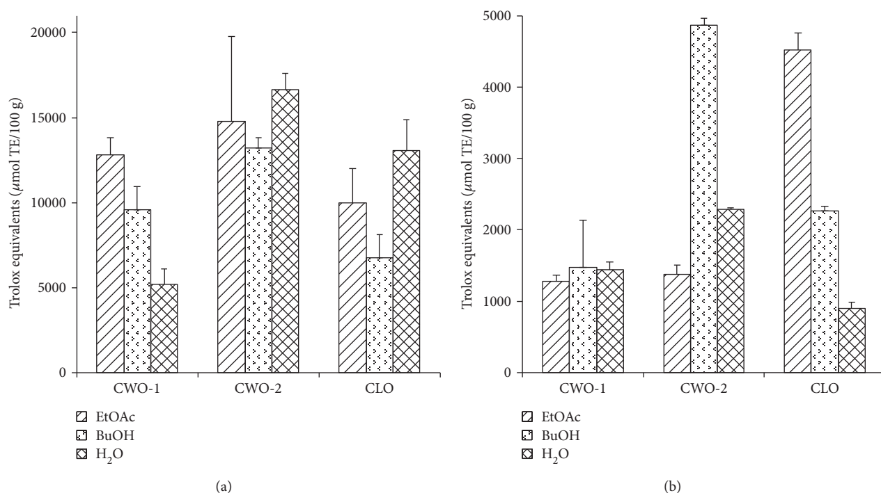
FIGURE 2: Antioxidative capacity in the extracts. CWO-1, CWO-2, and CLO which were sequentially extracted using EtOAc, BuOH, and water. The results are shown as Trolox equivalents ( \mu\text{mol TE}/100\text{ g} ). (a) ORAC assay with extract concentrations of 0.1 mg/ml. (b) FRAP assay with extract concentrations of 10 mg/ml. CWO = cold-pressed whale oil; CLO = cod liver oil; EtOAc = ethyl acetate; BuOH = butyl alcohol; ORAC = oxygen radical absorbance capacity; FRAP = ferric reducing antioxidant power.
