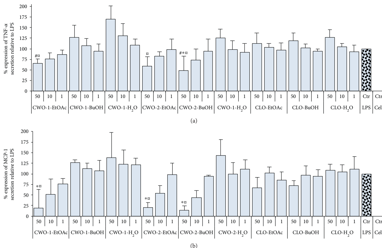
FIGURE 3: ELISA results for relative response of TNF- \alpha and MCP-1 in LPS-treated THP-1 cells. Each extract was tested at three different concentrations (50 \mu g/ml, 10 \mu g/ml, and 1 \mu g/ml), and the results are presented as mean with SD displayed as positive bars ( n = 3 ). (a) TNF- \alpha secretion relative to control. * p < 0.05 compared to LPS control. # p < 0.05 compared to CLO-BuOH 50 \mu g/ml. □ p < 0.05 compared to CLO-H 2 O 50 \mu g/ml. (b) MCP-1 secretion relative to control. * p < 0.001 compared to LPS control. # p < 0.001 compared to CLO-H 2 O 50 \mu g/ml. TNF- \alpha = tumor necrosis factor-alpha; MCP-1 = monocyte chemoattractant protein-1; LPS = lipopolysaccharide; CWO = cold-pressed whale oil; CLO = cod liver oil; EtOAc = ethyl acetate; BuOH = butyl alcohol.
