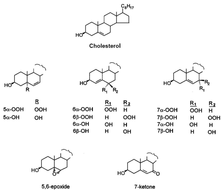
Fig. 2. Structures of cholesterol (cholest-5-en-3 \beta -ol), relevant cholesterol hydroperoxide positional isomers, and other cholesterol oxidation products. Identification of 5 \alpha -OOH, 6 \alpha -OOH, 6 \beta -OOH, and the corresponding alcohols signifies singlet oxygen involvement in a reaction. Identification of 7 \alpha -OOH, 7 \beta -OOH and their alcohols, along with 7-ketone and 5,6-epoxide, signifies free radical involvement.
