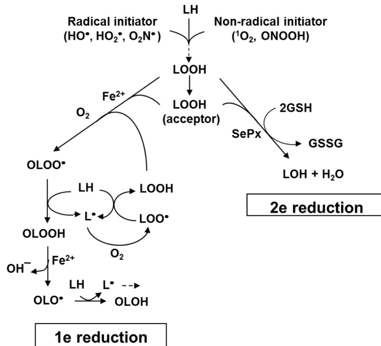
Fig. 1. Primary and secondary reactions of lipid peroxidation. Possible free radical and non-radical initiators are shown. Three different fates for LOOH intermediates are described: (i) iron-mediated one-electron reduction, resulting in chain amplification; (ii) selenoperoxidase (SePx)-catalyzed two-electron reduction, resulting in chain suppression; (iii) translocation to a membrane/lipoprotein acceptor where processes (i) or (ii) can take place.
