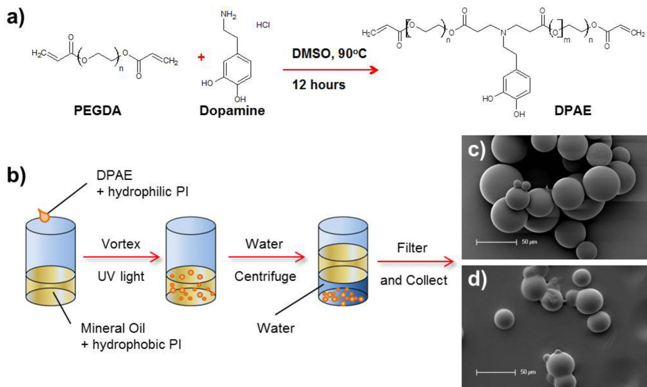
Figure 1. Formation of the dopamine containing poly( \beta -amino ester)(DPAE) via Michael type addition ( a ). This DPAE pre-polymer could then be emulsified in oil and photocrosslinked into beads ready for filtration and collection ( b ). SEM images show spherical beads formed from PEG ( c ) or DPAE ( d ).
