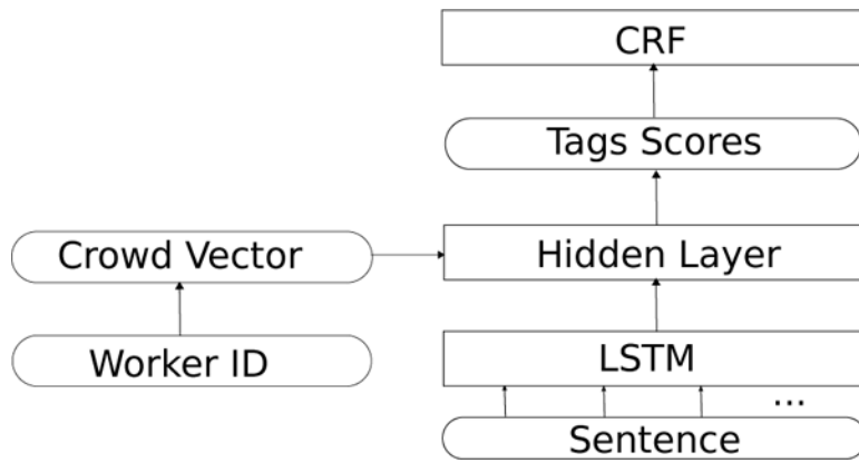
Figure 3. The LSTM-Crowd-cat model. The crowd vectors provide additional input for the Hidden Layer (they are effectively concatenated to the output of the LSTM block).
